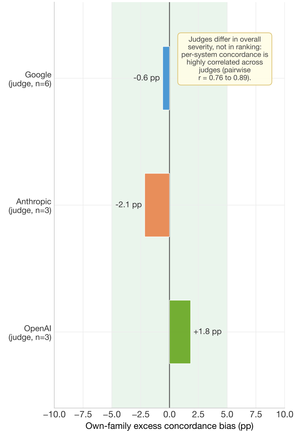
B Own-family bias after removing judge severity
