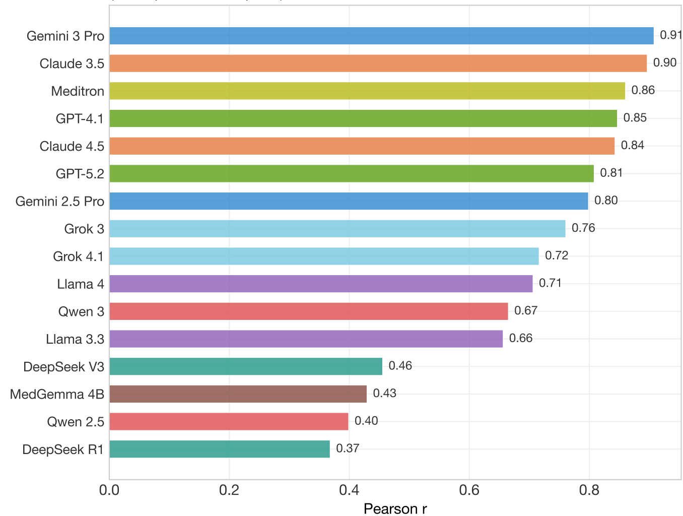
A Test-Retest Correlation (92 duplicate case pairs)
