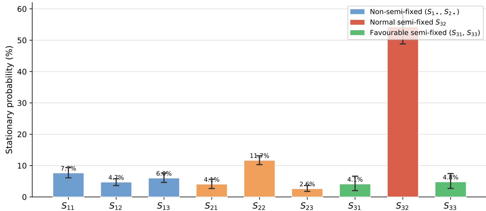
Stationary distribution of the 9-state Markov chain (bars = point estimates; whiskers = 95% bootstrap CI, B=2000)
