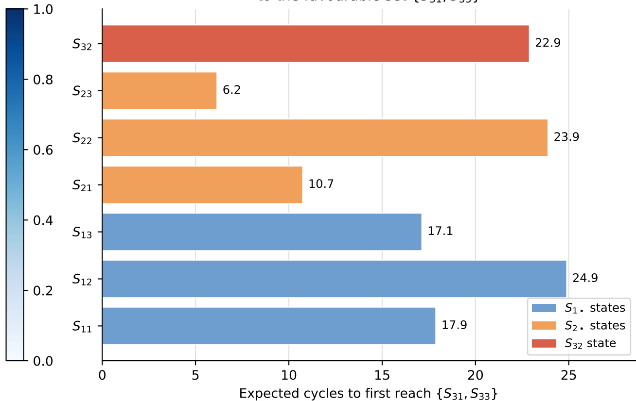
Mean first passage time (MFPT) to the favourable set \{S_{31}, S_{33}\}
