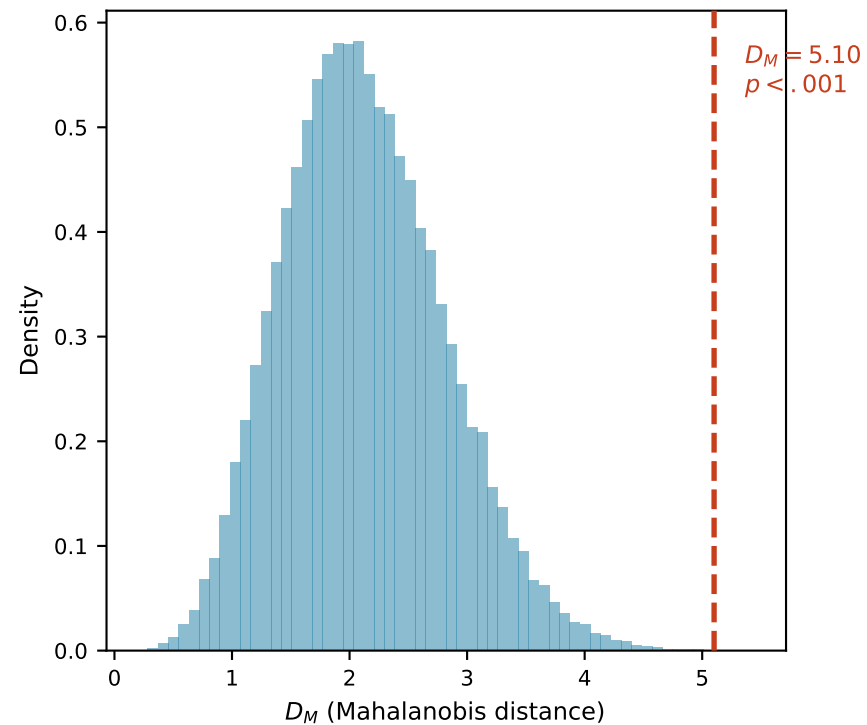
Permutation ( H_G ) null
