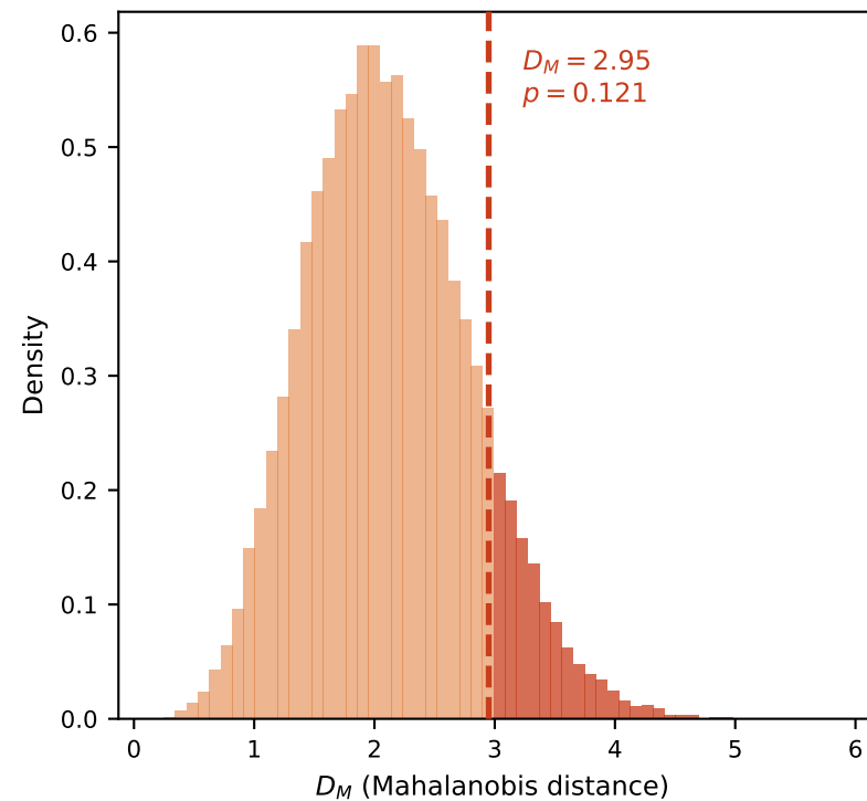
Within-woman ( H_W ) null
