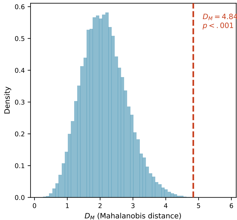
Multinomial ( H_{id} ) null
