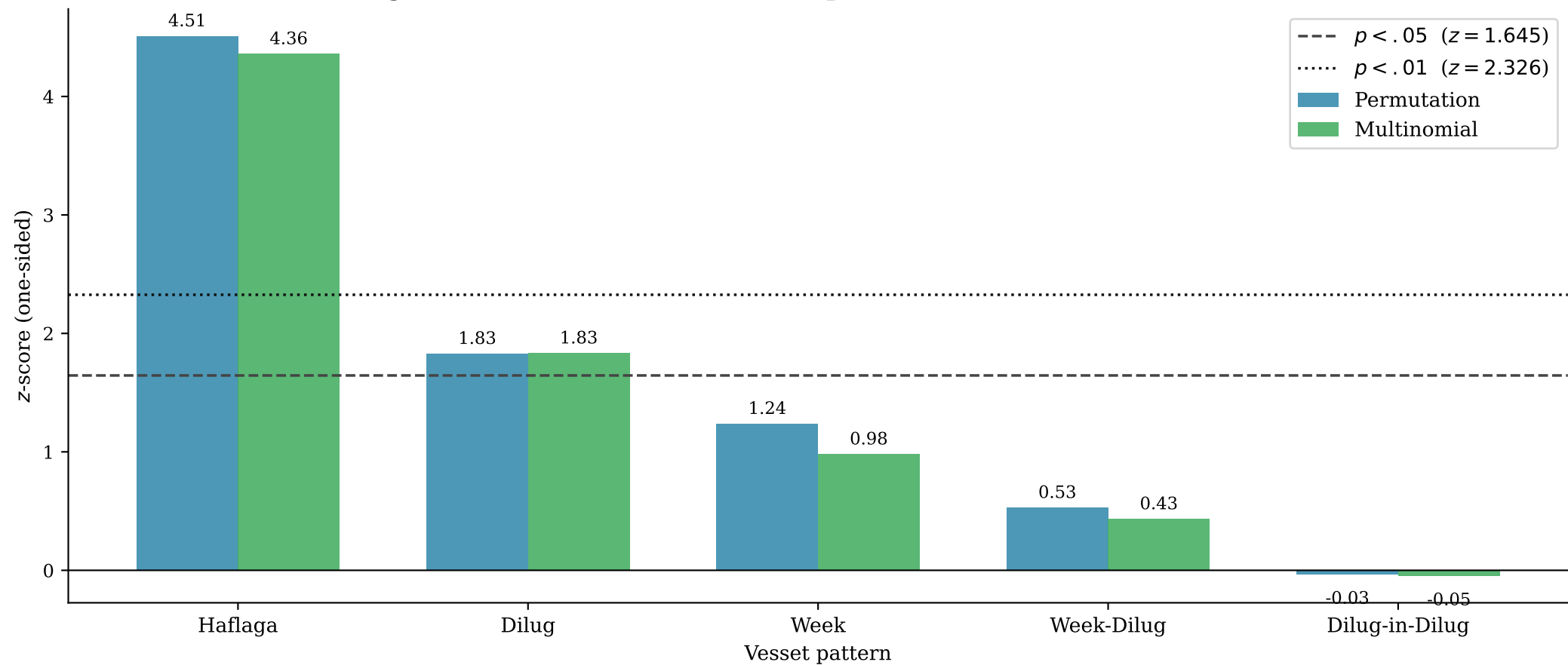
Figure 2. Effect sizes (z-scores) — permutation vs. multinomial null
