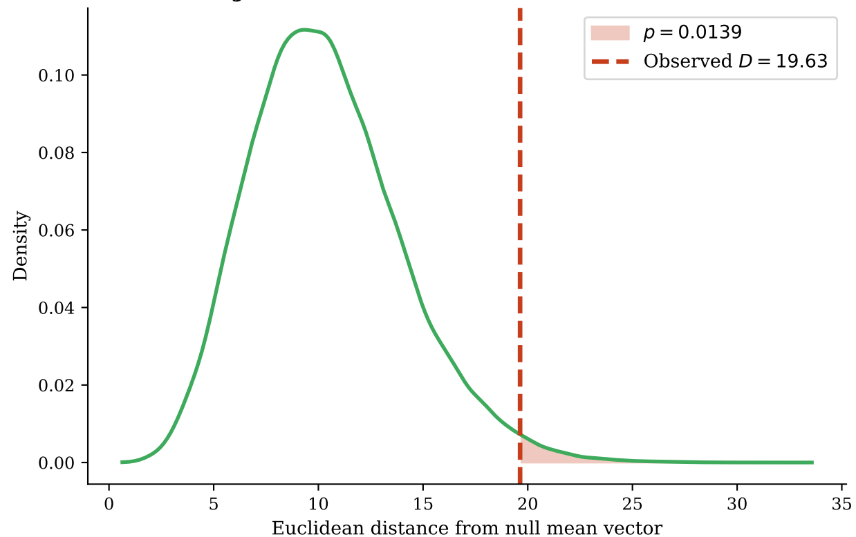
Figure 3. Joint multivariate test (all 5 patterns) (shaded area = p-value region)
