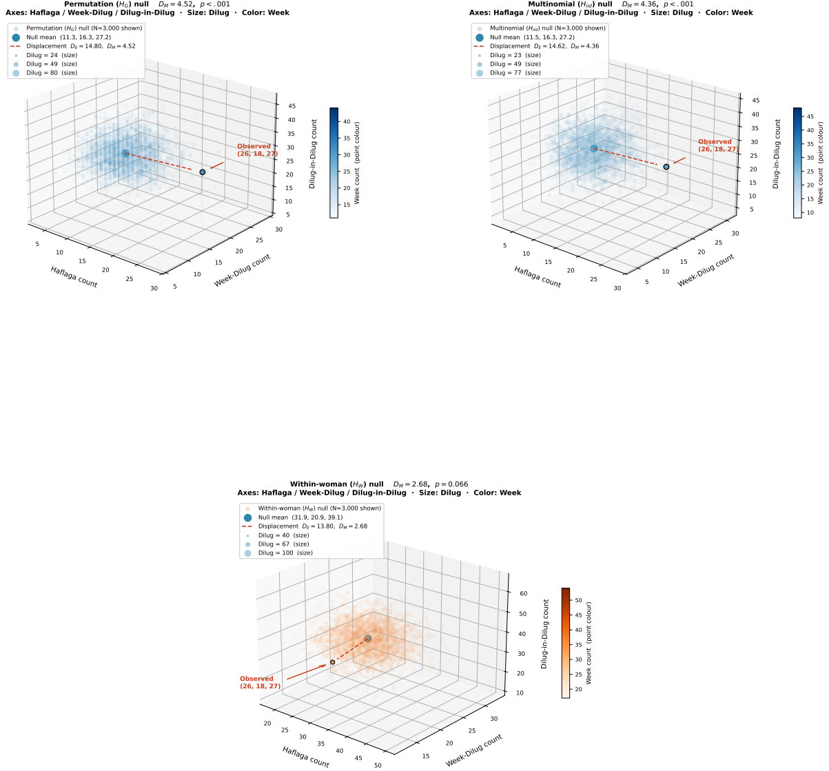
Figure 9: Exploratory focused subspace analysis: displacement of the observed count vector (26, 18, 27) in the (Haftaga, Week-Dilug, Dilug-in-Dilug) subspace under the permutation ( H_G , top left), multinomial ( H_{iid} , top right), and within-woman ( H_W , bottom centre) nulls. Marker size encodes Dilug count; marker shading encodes Week count. The filled circle marks the null mean; the dashed line identifies the displacement. Under H_G and H_{iid} the observed vector lies at the periphery of the null cloud (3-pattern D_M = 4.52 and 4.36 , both p < .001 ; primary 5-pattern D_M = 5.10 and 4.84 ). Under H_W the observed vector falls within the null cloud (3-pattern D_M = 2.68 , p = .066 ; primary 5-pattern D_M = 2.95 , p = .121 ; Table 3). This figure is an exploratory geometric complement to the primary 5-pattern analysis.
