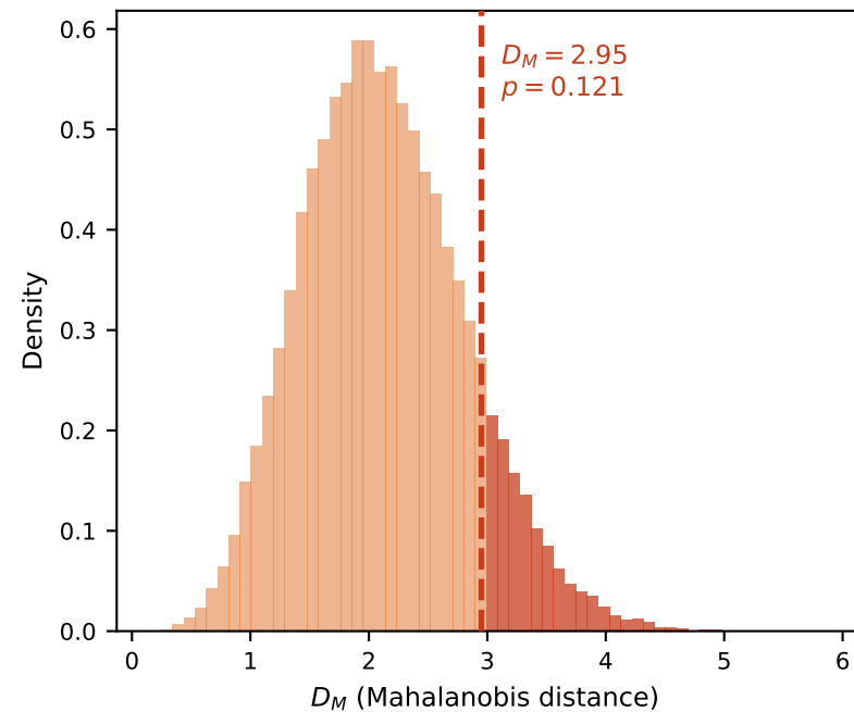
Within-woman ( H_W ) null
