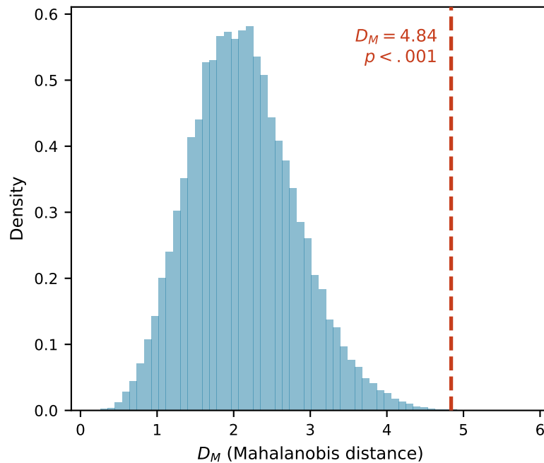
Multinomial ( H_{iid} ) null
