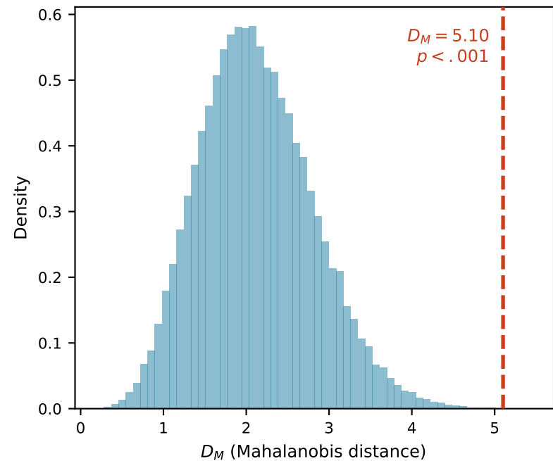
Permutation ( H_G ) null
