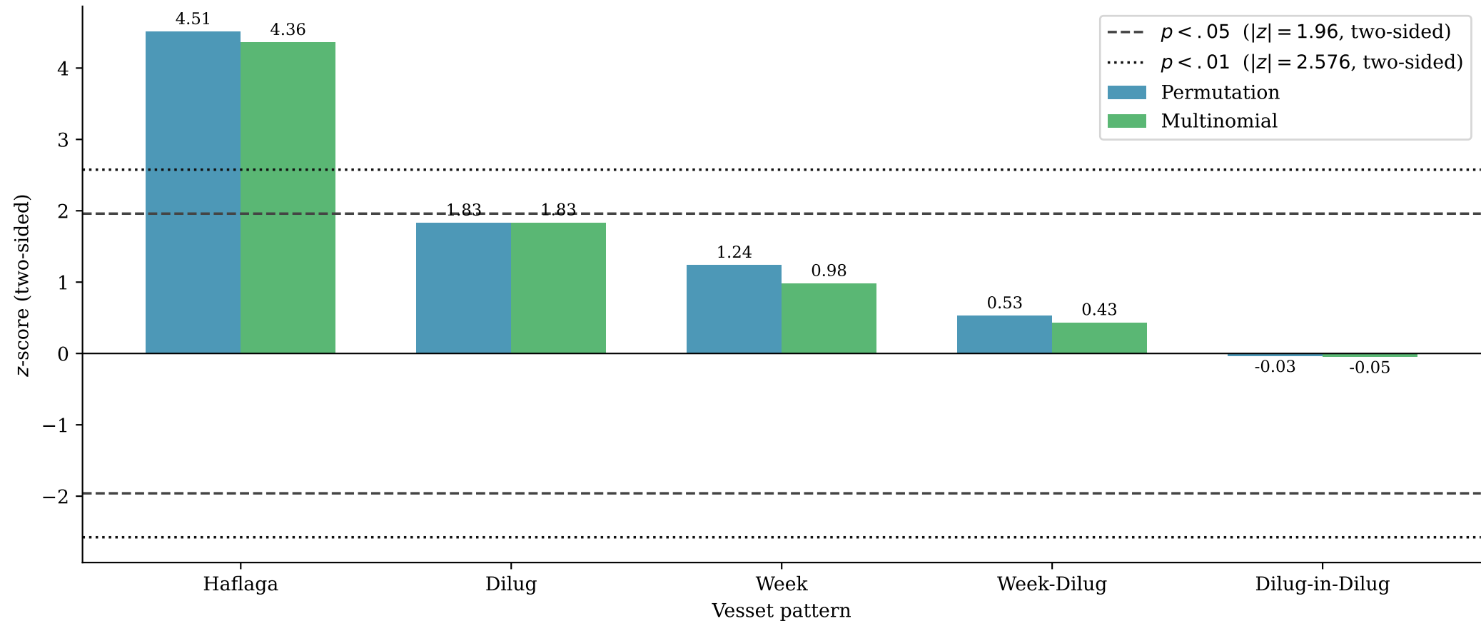
Figure 4. Effect sizes (z-scores) — permutation vs. multinomial null
