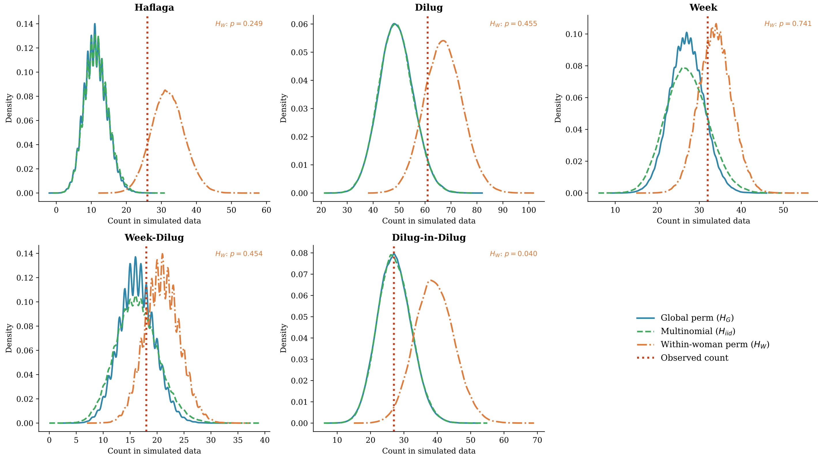
Figure 6. Null distributions ( H_G , H_{iid} , H_W ) vs. observed counts Global null: joint D_M = 5.10 , p < .001 | Within-woman null (primary): D_M = 2.95 , p = .121 | H_W two-sided p -values shown per panel
