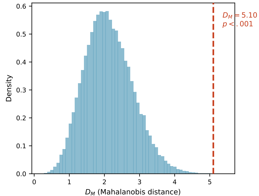
Permutation ( H_G ) null
