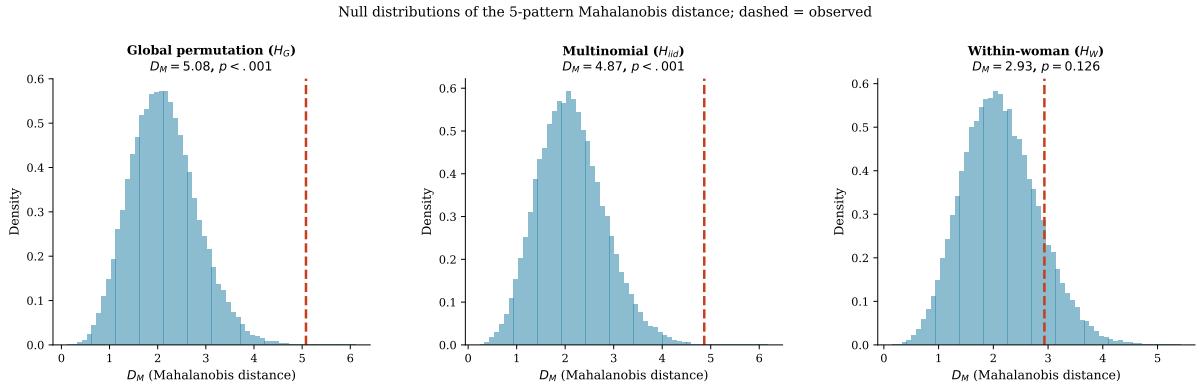
Figure 6: Null distributions of the five-pattern Mahalanobis distance D_M (Eq. 2) under H_G (left), H_{iid} (centre) and H_W (right); dashed line at the observed value.
