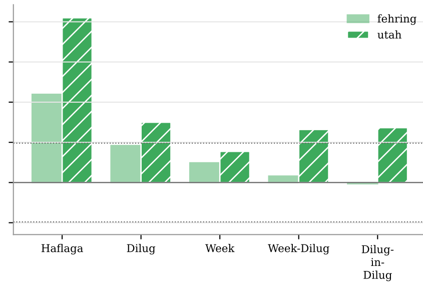
Multinomial ( H_{iid} ) D_M 4.87 ( p < .001 ) vs 9.56 ( p < .001 )
