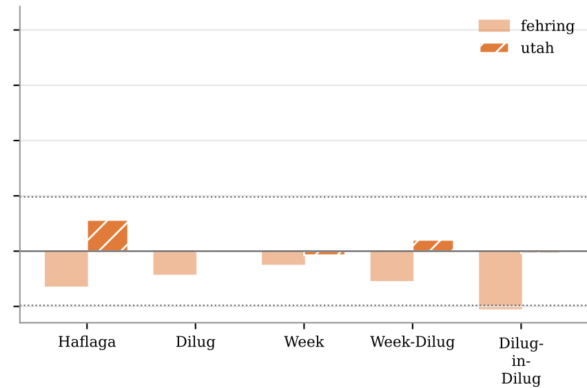
Within-woman permutation ( H_W ) D_M 2.97 ( p = 0.115 ) vs 1.22 ( p = 0.916 )
