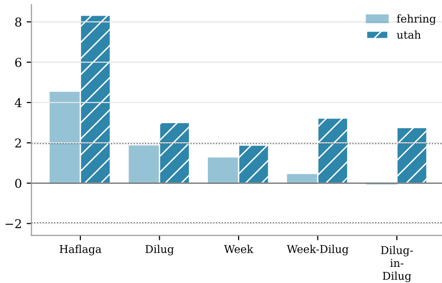
Global permutation ( H_G ) D_M 5.07 ( p < .001 ) vs 10.04 ( p < .001 )
