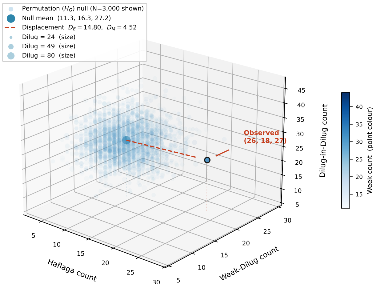
Permutation ( H_G ) null D_M = 4.52 , p < .001 Axes: Haflaga / Week-Dilug / Dilug-in-Dilug · Size: Dilug · Color: Week
