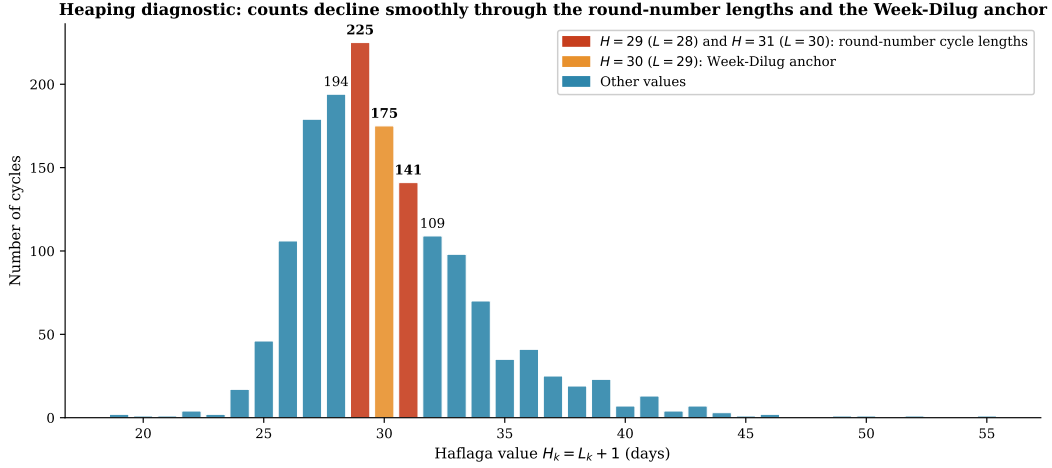
Figure 10: Frequency of each interval value H_k = L_k + 1 in the analysed sample. Red bars: H = 29 and H = 31 , the round-number cycle lengths L = 28 and L = 30 at which digit preference would appear; orange bar: H = 30 ( L = 29 ), the Week-Dilug anchor. Counts decline smoothly through these values (225, 175, 141), so the Week-Dilug count does not appear to reflect reporting heaping.
