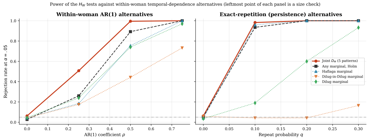
Figure 8: Rejection rates of the H_W tests at \alpha = .05 against within-woman AR(1) alternatives (left) and exact-repetition alternatives (right); the leftmost point of each panel is a size check. Solid: joint five-pattern D_M ; dashed: any Holm-corrected marginal; dotted: selected marginal tests. Dash-dotted horizontal line at 0.05.
