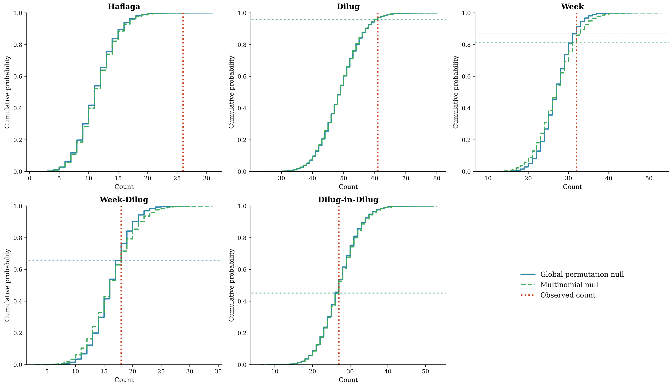
Empirical CDFs of the global null distributions (horizontal dotted = F(O - 1) )
