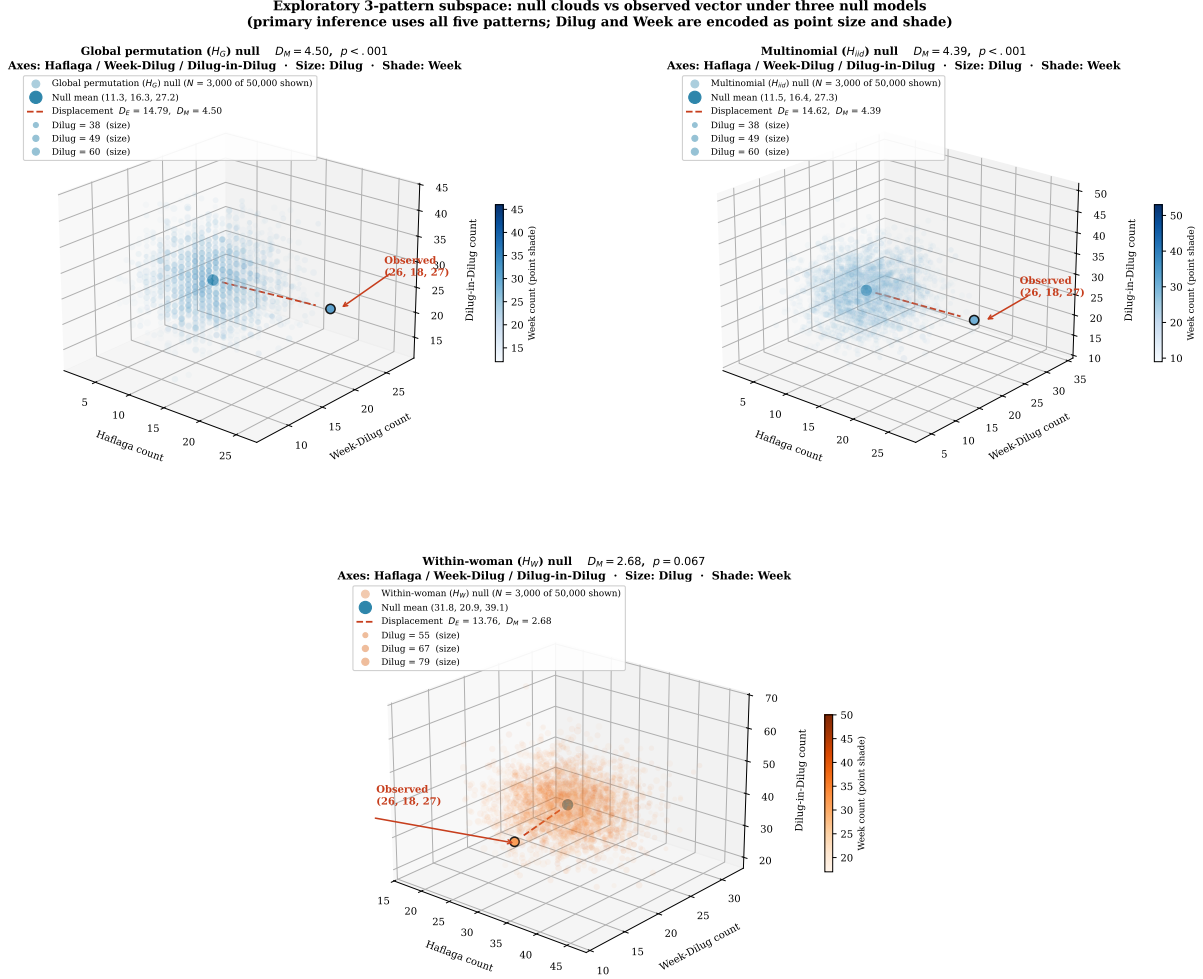
Figure 8: Exploratory three-pattern subspace: 3,000 of the 50,000 null replicates (points) and the observed vector (26, 18, 27) in the (Haflaga, Week-Dilug, Dilug-in-Dilug) space under H_G (top left), H_{iid} (top right) and H_W (bottom), so that all five counts are visible at once: marker size encodes the Dilug count (size legend in each panel) and marker shade the Week count (colour bar). The filled circle is the null mean; the dashed segment is the displacement to the observed vector, with its Euclidean length D_E and Mahalanobis length D_M in the legend. Primary inference uses all five patterns (Table 3).
