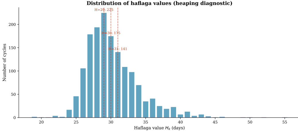
Figure 11: Frequency of each haflaga value H_k in the analysed sample. Counts decline smoothly across the Week-Dilug anchor ( H = 29: 225; 30: 175; 31: 141 ).
