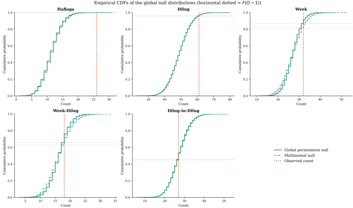
Figure 5: Empirical CDFs of the H_G (solid) and H_{iiid} (dashed) null distributions; dotted vertical line at the observed count.
