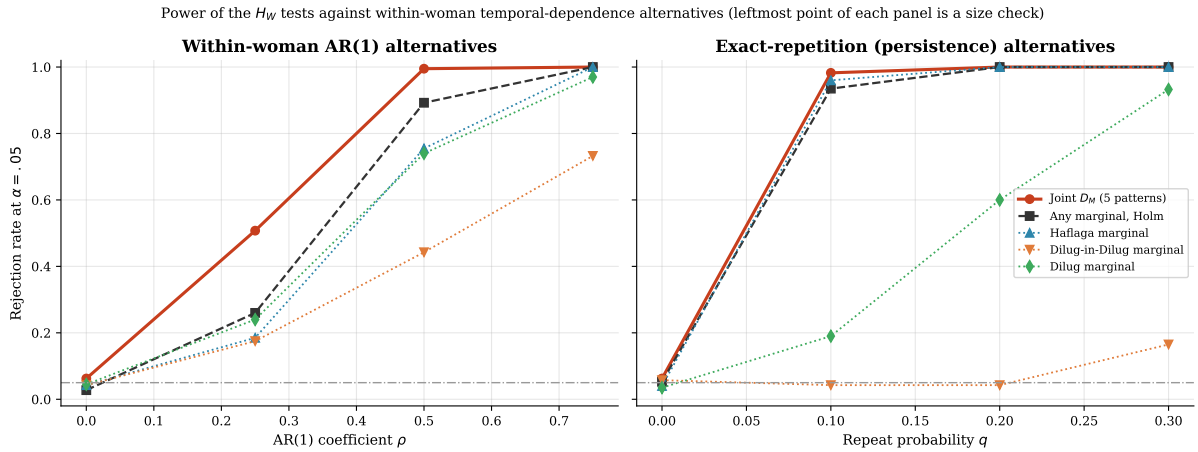
Figure 10: Rejection rates of the H_W tests at \alpha = .05 against within-woman AR(1) alternatives (left) and exact-repetition alternatives (right); the leftmost point of each panel is a size check. Solid: joint five-pattern D_M ; dashed: any Holm-corrected marginal; dotted: selected marginal tests. Dash-dotted horizontal line at 0.05.
