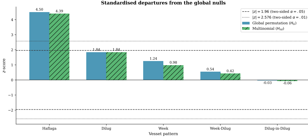
Figure 4: Standardised departures z_j under H_G (solid) and H_{iiid} (hatched). Dashed and dotted lines mark |z| = 1.96 and 2.576 . The two nulls give different z for the same count because each has its own mean and SD (e.g. Week: 1.24 vs. 0.98).
