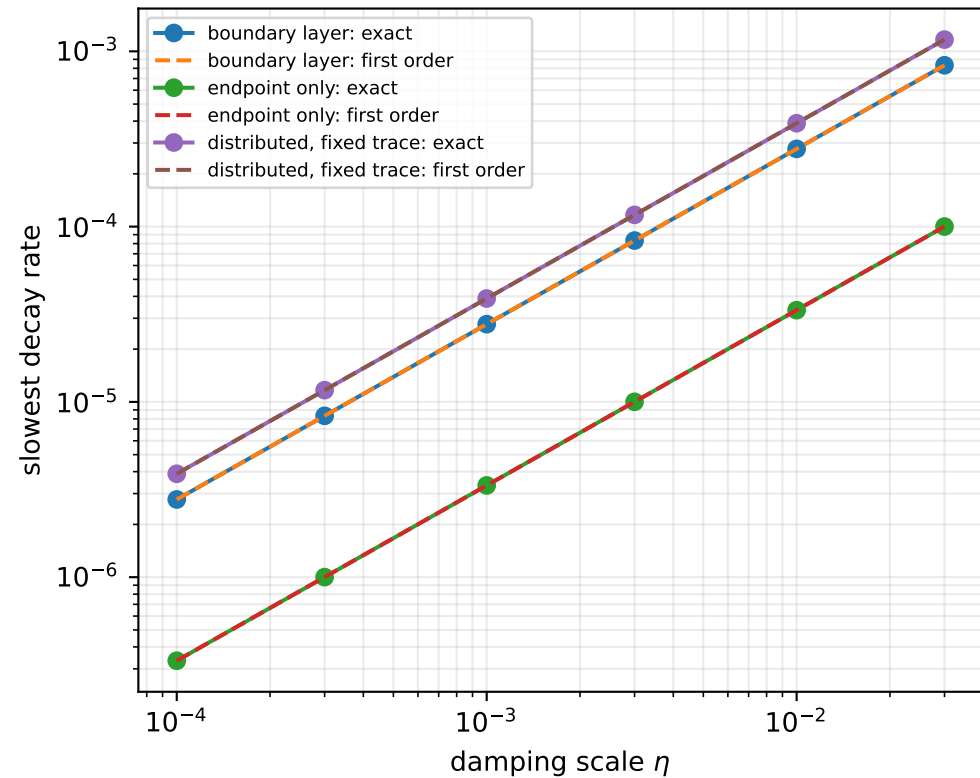
Weak-damping modal law
