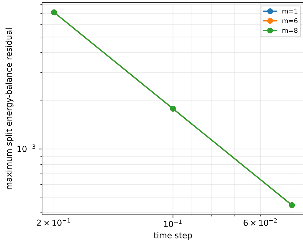
Integration consistency
