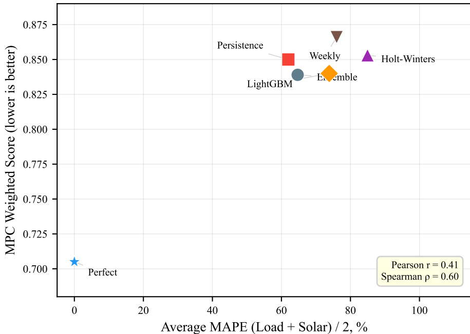
Forecast Quality (MAPE) vs. Control Performance (MPC Score)
