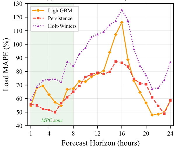
(a) Load Forecast Error by Horizon
