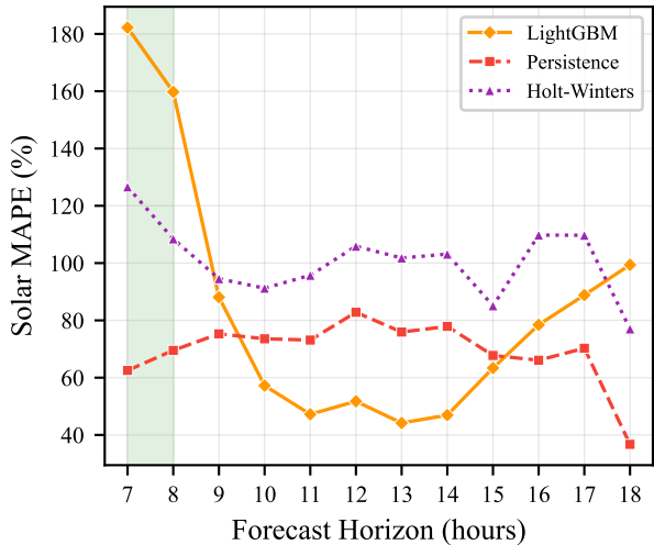
(b) Solar Forecast Error by Horizon (daylight only)
