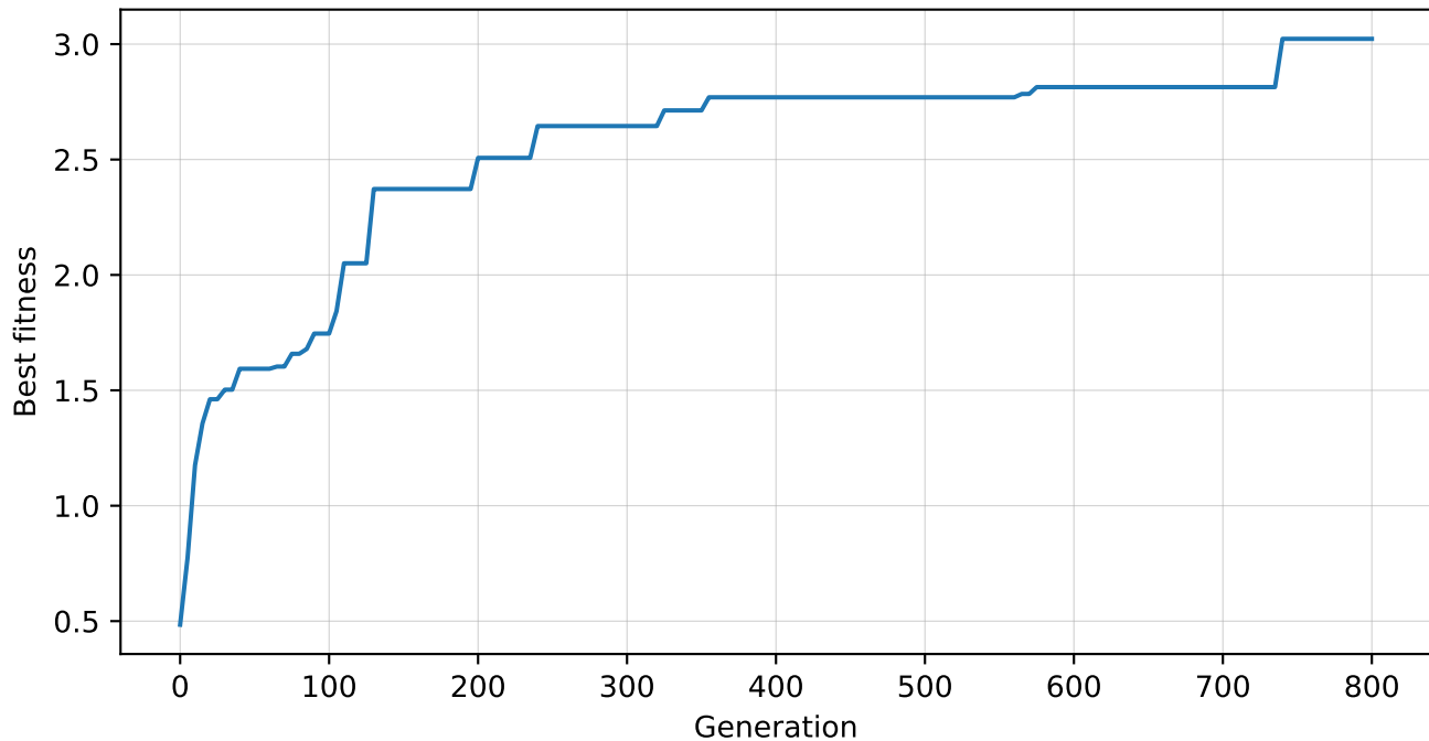
Best fitness over generations
