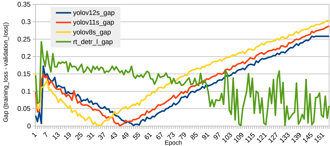
Training-Validation loss gap
