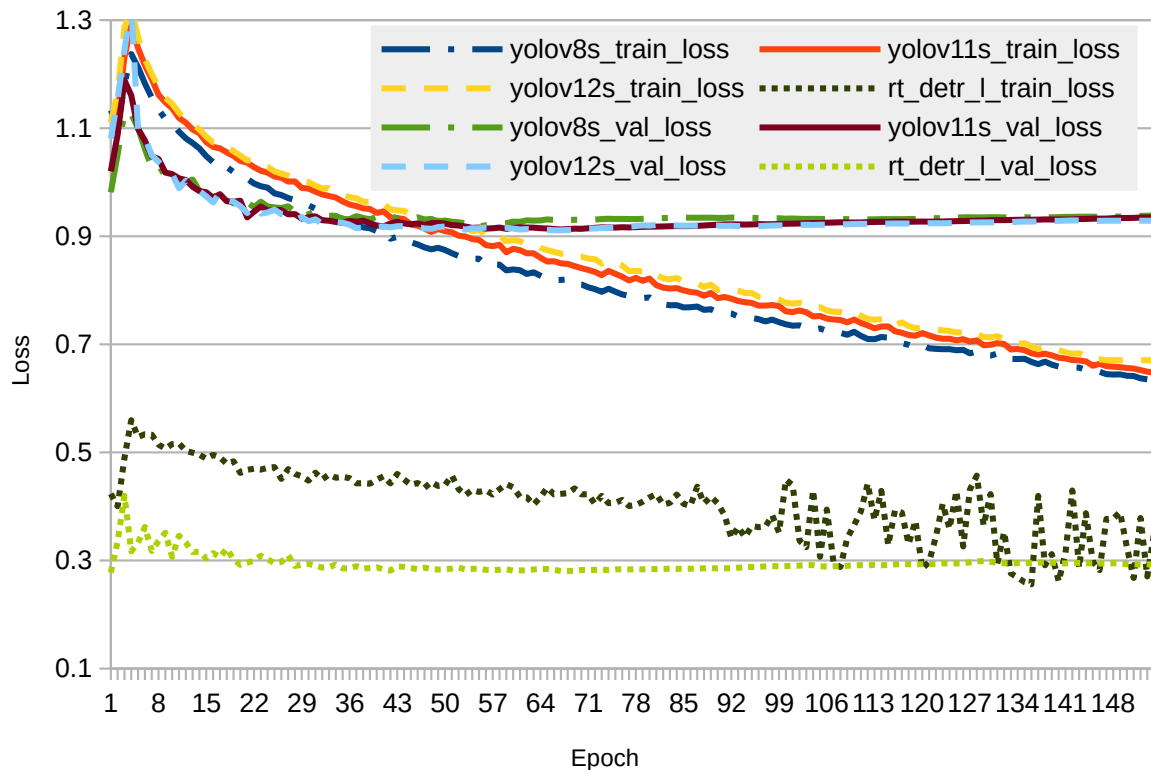
Training and validation loss graphs
