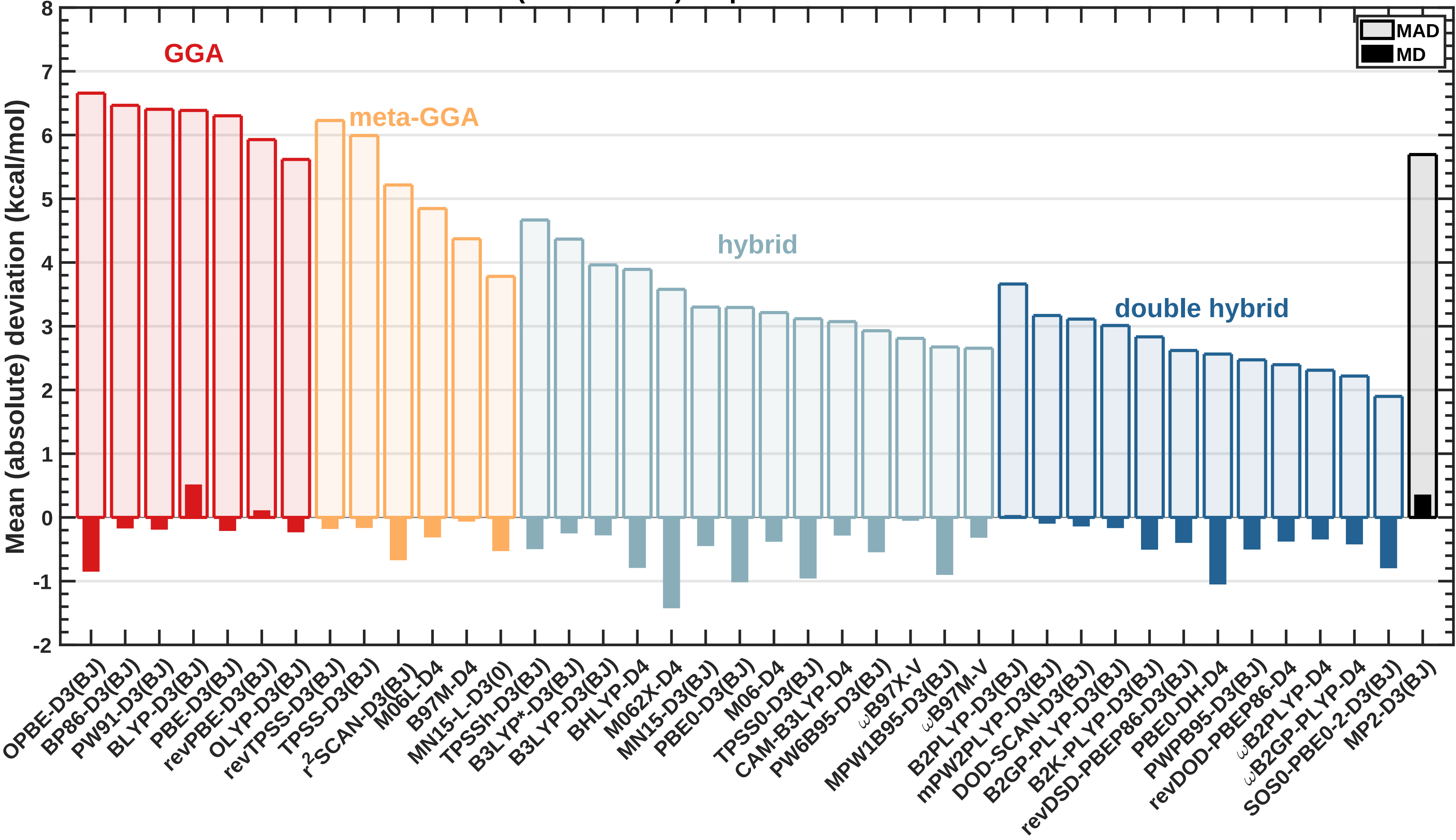
Results for the best (lowest MAD) dispersion corrected variant of each method
