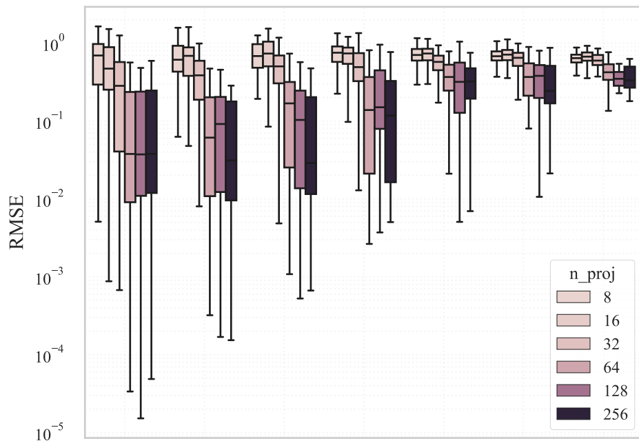
Skew Covariance Error \|\mathbf{U}^* - \widehat{\mathbf{U}}\|_F
