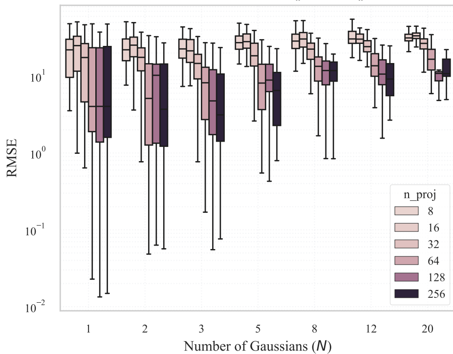
Skew Covariance Error \|\mathbf{U}^* - \widehat{\mathbf{U}}\|_F
