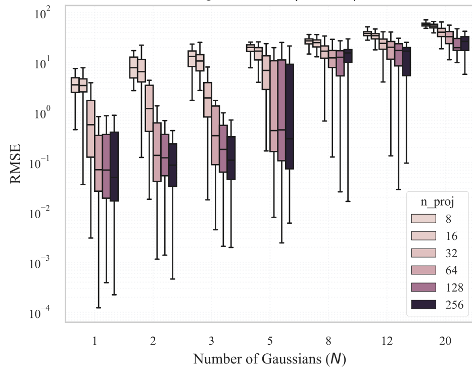
Amplitude Error |\alpha^* - \widehat{\alpha}|
