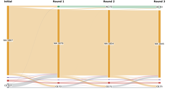
Fig. 3. Verdict transitions of all 2,076 proxy-model bugs across the three self-reflection rounds. The accepted (green) band grows only 0 → 53 → 73 → 83; wrong answers dominate and persist, and runtime/time-limit failures never resolve.
