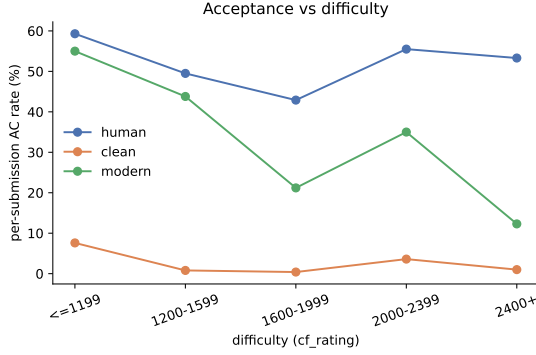
Fig. 3. Acceptance vs. difficulty: the proxy model is at the floor, the modern model declines overall but not monotonically, and humans are flat (survivorship).
