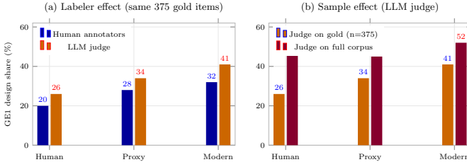
Fig. 2. Deconfounding the apparent design (GE1) reversal. (a) Holding the sample fixed (the same 375 gold items), the LLM judge inflates the design family ( \sim +6-9 points) but preserves the human<proxy<modern ordering—its granularity bias is a level shift, not a reversal. (b) Holding the labeler fixed (judge), moving from the stratified gold to the full corpus changes the ordering (proxy drops to last): the “reversal” is a sample effect. Neither route yields a robustly ordered difference.
