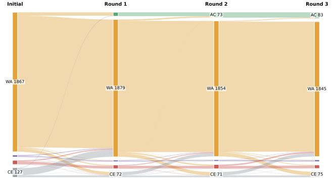
Fig. 4. Verdict transitions of all 2,076 proxy-model bugs across the three self-reflection rounds. The accepted (green) band grows only 0 \rightarrow 53 \rightarrow 73 \rightarrow 83; wrong answers dominate and persist, and runtime/time-limit failures never resolve.
