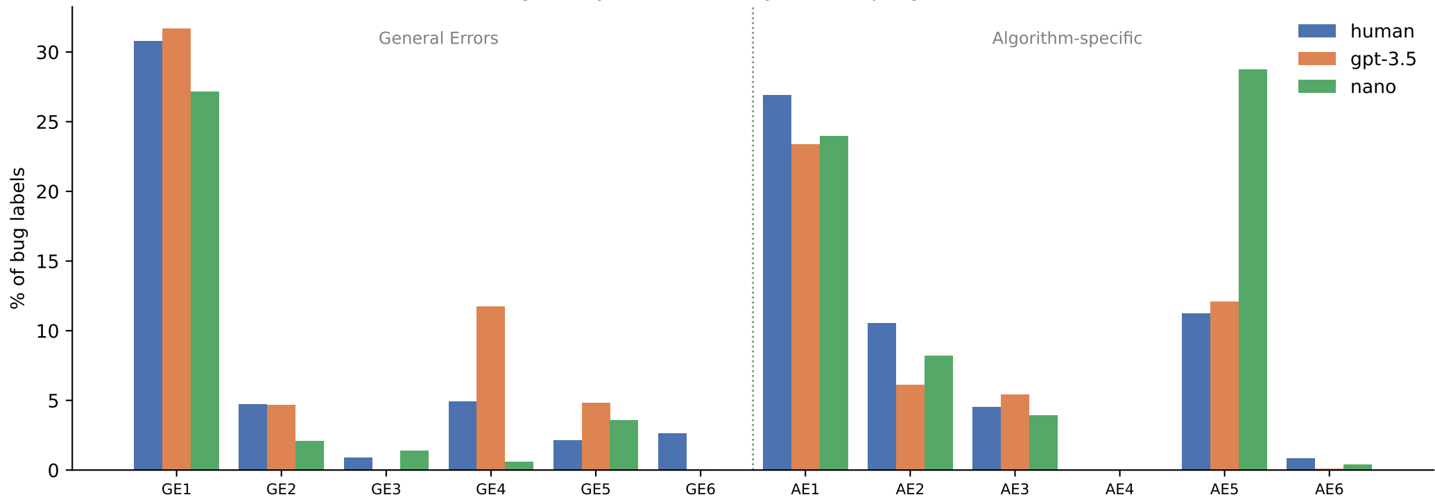
Bug-family distribution by author (judge labels)
