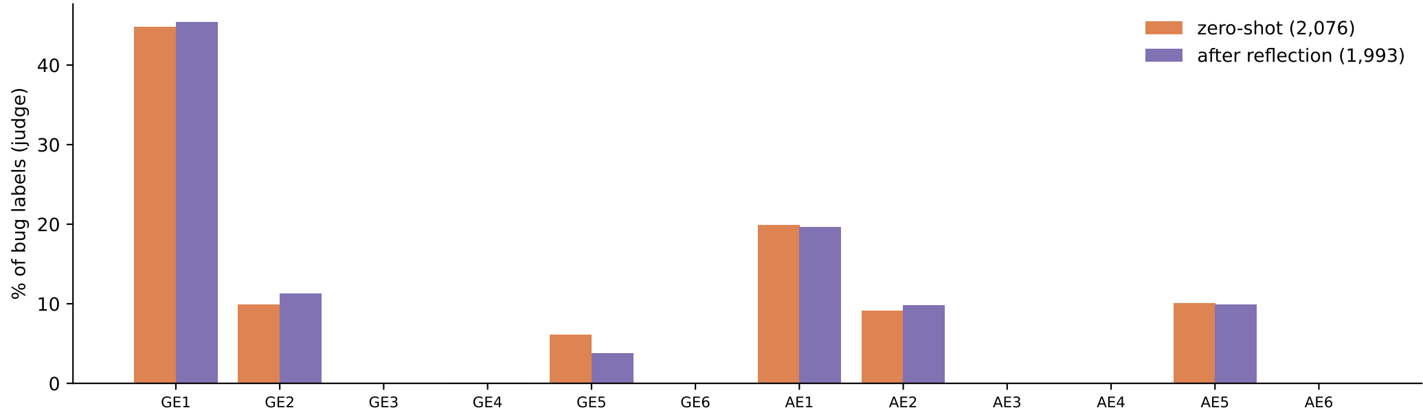
Clean-model bug families: before vs after self-reflection
