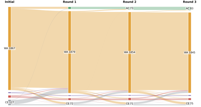
Fig. 4. Verdict transitions of all 2,076 proxy-model bugs across the three self-reflection rounds. The accepted (green) band grows only 0 \rightarrow 53 \rightarrow 73 \rightarrow 83; wrong answers dominate and persist, and runtime/time-limit failures never resolve.
