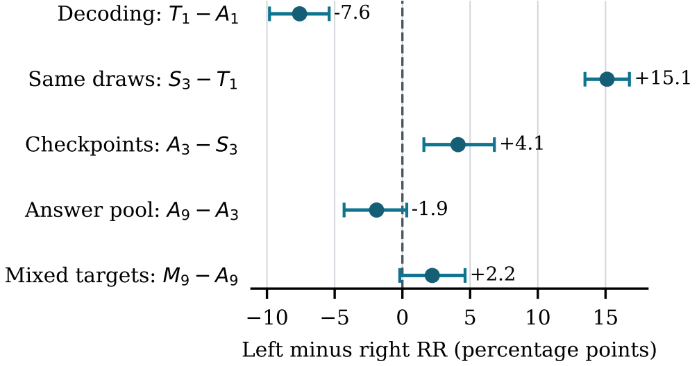
Fig. 2. Adjacent Seen RR contrasts in the mechanism ladder (problem-cluster 95% CIs). Absolute RR for A_1, T_1, S_3, A_3, A_9, M_9 is respectively 50.1, 42.5, 57.6, 61.7, 59.8, and 61.5%. The first three contrasts use exactly the same three stochastic candidates; the final contrast is five-fold problem-cross-fitted.
