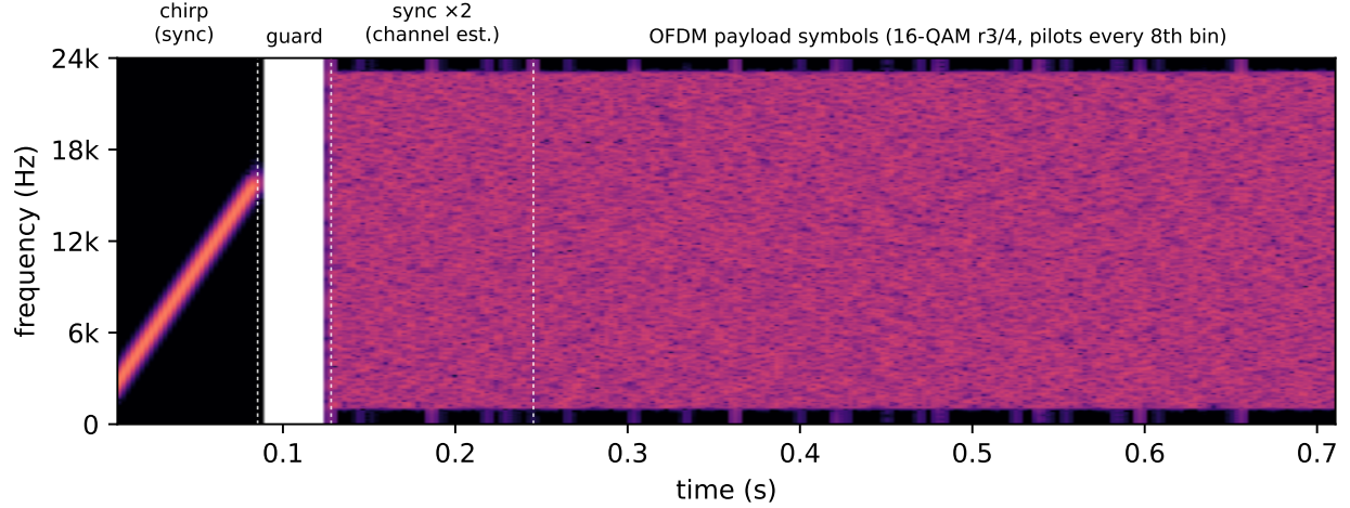
Figure 2: Spectrogram of one transmitted bulk-PHY frame (generated by the reference modem, 16-QAM rate 3/4, 8 data symbols): a 2→16 kHz linear chirp for coarse synchronization, a guard gap so the chirp’s reverberant tail decays, two known full-band OFDM symbols for channel estimation, then the OFDM payload symbols spanning 1.1–23 kHz with comb pilots on every 8th subcarrier. Over the air this sounds like a short chirp followed by a breath of static; the static is the data.
