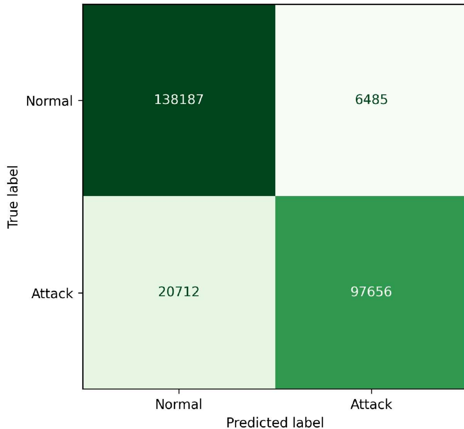
Ensemble Confusion Matrix
