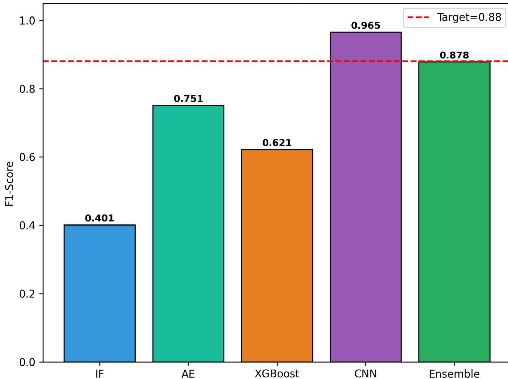
F1-Score Across Pipeline Layers
