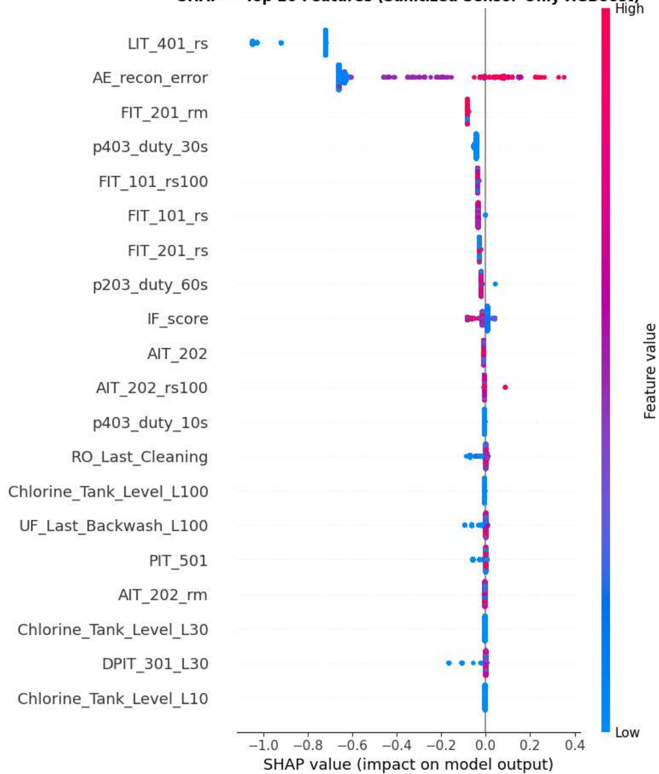
SHAP — Top 20 Features (Sanitized Sensor-Only XGBoost)
