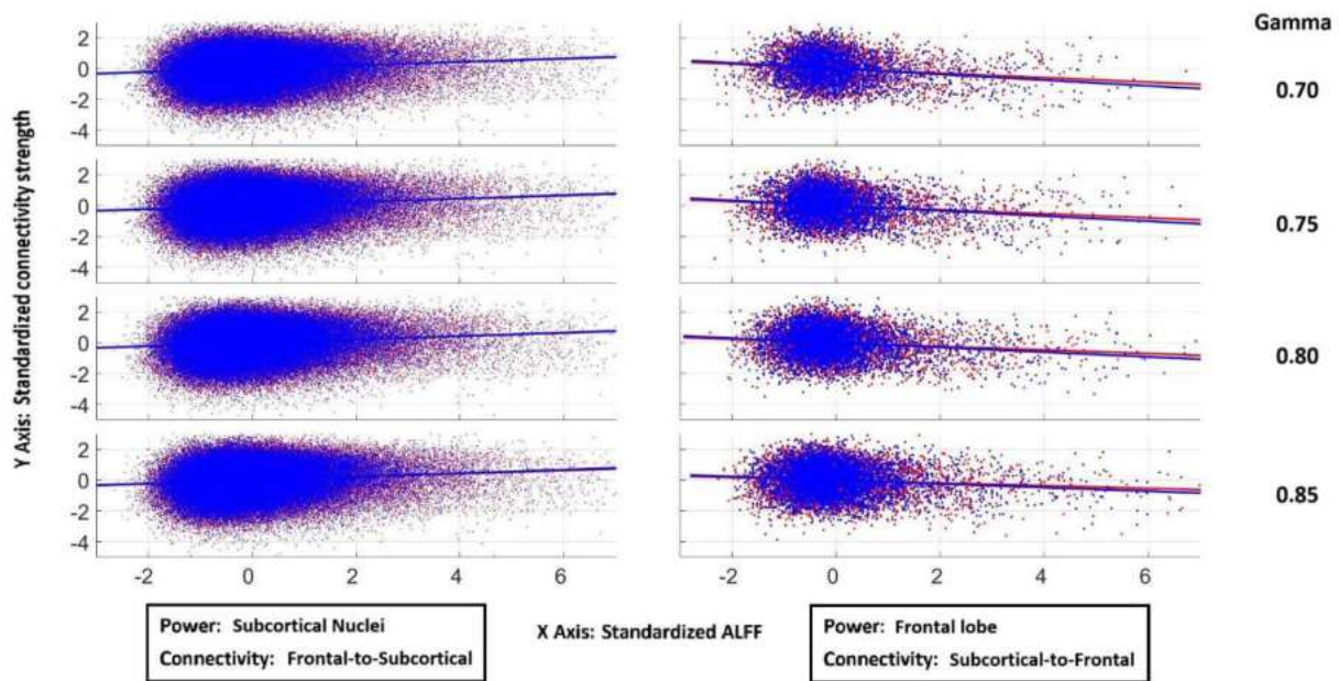
Figure 3. Scatter plots with regression lines illustrating the relationships between regional power and functional connectivity. Left column: voxel-wise ALFF within subcortical nuclei plotted against mean frontal-to-subcortical nodal strength. Right column: mean ALFF within the frontal lobe plotted against mean subcortical-to-frontal nodal strength. Rows correspond to four increasing Gamma values (0.70 to 0.85). The left and right columns show robust but opposing trends, as reflected in the opposite directions of the regression slopes. Blue indicates HC, and red indicates ADHD.
