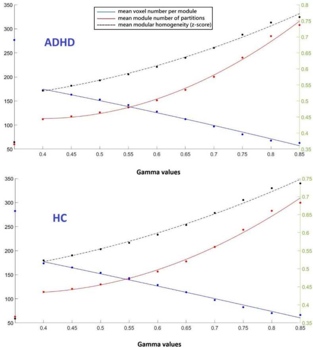
Figure 2. Scatter plots showing three metrics derived from the ADHD200 dataset across 10 gamma values (X-axis), with second-order polynomial regression curves overlaid. Each plot contains 10 data points per metric, corresponding to the tested gamma values. The top panel illustrates results for the ADHD group, while the bottom panel shows those for the HC group. The point at x = 0 denotes the initial parcellation using the Desikan-Killiany atlas. Red markers and curves represent the mean number of modules (left Y-axis), blue markers and curves indicate the average voxel count per module (left Y-axis), and black markers and curves denote the mean within-module z-score (right Y-axis), reflecting modular homogeneity.
