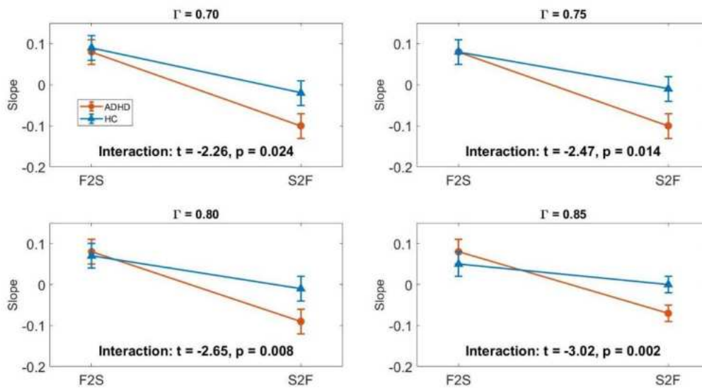
Figure 4. Relationships between ALFF and nodal strength in the NAc and frontal lobe based on slopes derived from Linear Mixed Effects (LME) models at four Gamma values. F2S: slopes of ALFF at NAc against mean functional connectivity between NAc and frontal lobe. S2F: slopes of mean ALFF at frontal lobe against mean functional connectivity between NAc and frontal lobe. Data are shown for two groups, ADHD (triangles) and HC (circles), with error bars representing standard errors. Interaction effects between group and condition are reported below each subplot.
