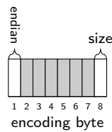
Figure 9.26: Encoding byte
