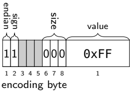
Figure 9.31: one byte big-endian value -255
