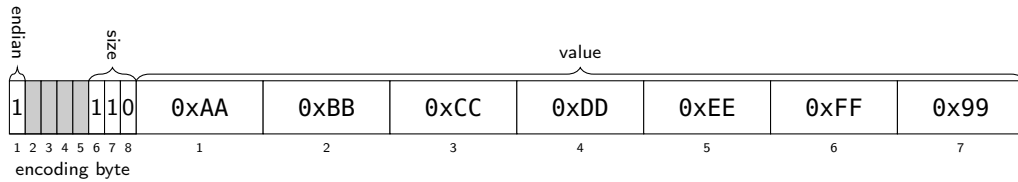
Figure 9.14: Dwm::EncodedU64 example: value 0xAABBCCDDEEFF99, big-endian.
