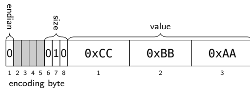
Figure 9.7: Dwm::EncodedU64 example: value 0xAABBCC, little-endian.
