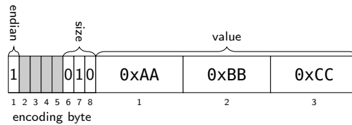
Figure 9.6: Dwm::EncodedU64 example: value 0xAABBCC, big-endian.
