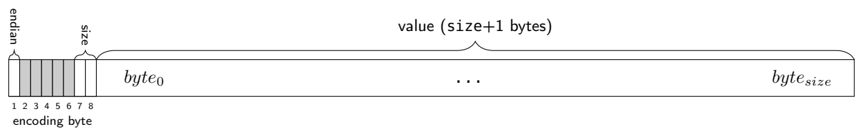
Figure 9.18: Dwm::EncodedU32 encoding
