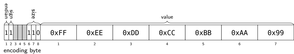
Figure 9.41: seven byte big-endian value -72,038,755,451,251,353
