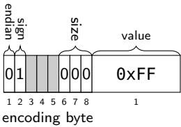
Figure 9.32: one byte little-endian value -255
