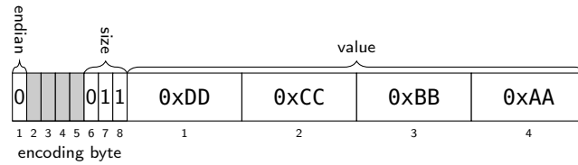
Figure 9.9: Dwm::EncodedU64 example: value 0xAABBCCDD, little-endian.
