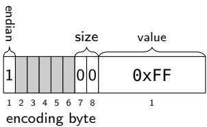
Figure 9.19: one byte big-endian value 255
