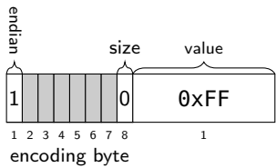
Figure 9.27: one byte big-endian value 255
