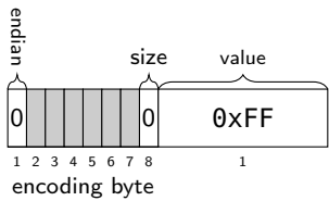
Figure 9.28: one byte little-endian value 255
