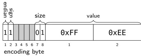
Figure 9.48: two byte big-endian value -65,518
