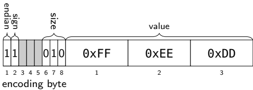
Figure 9.34: three byte big-endian value -16,772,829
