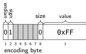
Figure 9.54: one byte little-endian value -255
