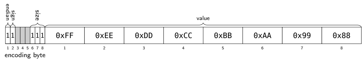
Figure 9.43: eight byte big-endian value -18,441,921,395,520,346,504
