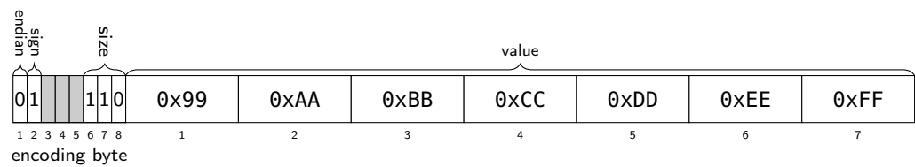
Figure 9.42: seven byte little-endian value -72,038,755,451,251,353
