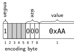
Figure 9.2: Dwm::EncodedU64 example: value 0xAA, big-endian.
