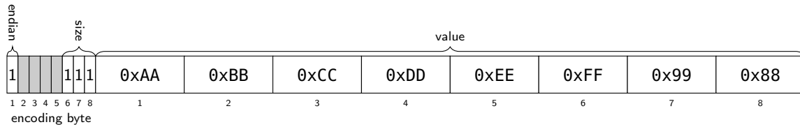
Figure 9.16: Dwm::EncodedU64 example: value 0xAABBCCDDEEFF9988, big-endian.
