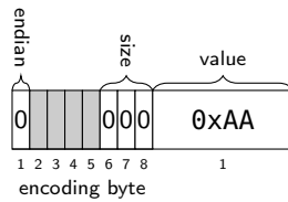
Figure 9.3: Dwm::EncodedU64 example: value 0xAA, little-endian.
