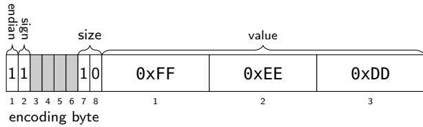
Figure 9.49: three byte big-endian value -16,772,829
