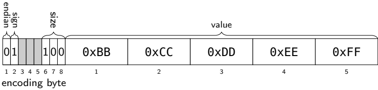
Figure 9.38: five byte little-endian value -1,099,224,173,755
