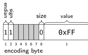
Figure 9.53: one byte big-endian value -255
