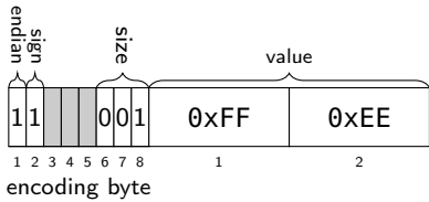
Figure 9.33: two byte big-endian value -65,518
