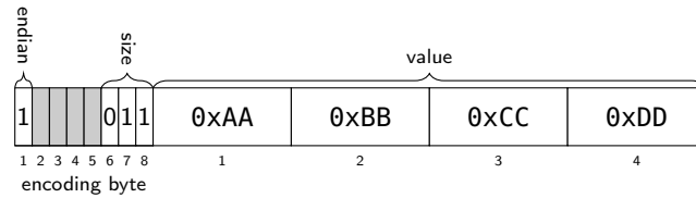
Figure 9.8: Dwm::EncodedU64 example: value 0xAABBCCDD, big-endian.
