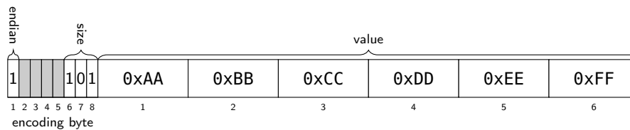
Figure 9.12: Dwm::EncodedU64 example: value 0xAABBCCDDEEFF, big-endian.
