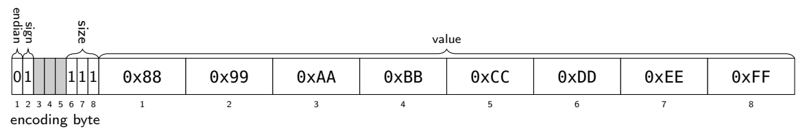
Figure 9.44: eight byte little-endian value -18,441,921,395,520,346,504
