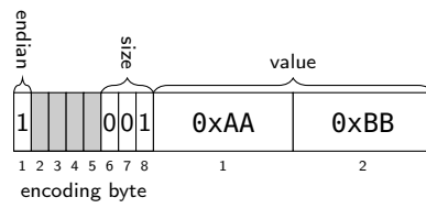
Figure 9.4: Dwm::EncodedU64 example: value 0xAABB, big-endian.
