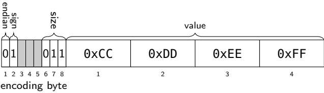
Figure 9.36: four byte little-endian value -4,293,844,428
