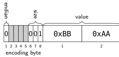
Figure 9.5: Dwm::EncodedU64 example: value 0xAABB, little-endian.
