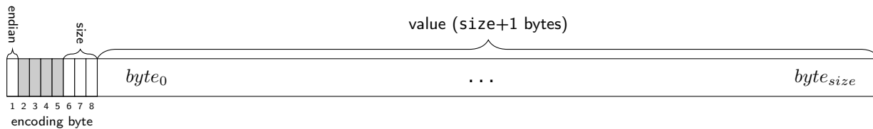
Figure 9.1: Dwm::EncodedU64 encoding
