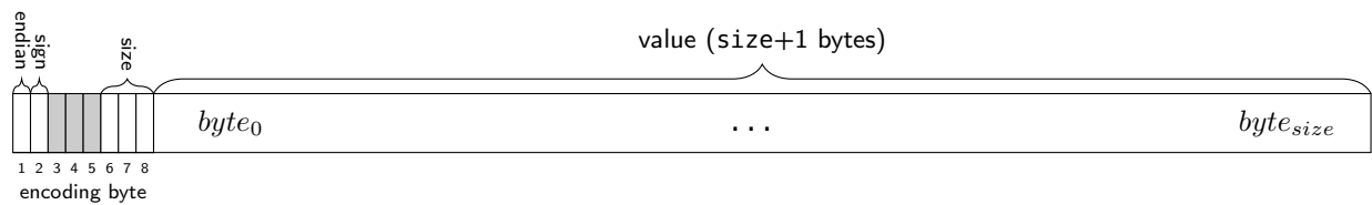
Figure 9.30: Dwm::EncodedS64 encoding
