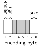
Figure 9.45: Encoding byte
