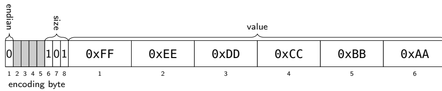
Figure 9.13: Dwm::EncodedU64 example: value 0xAABBCCDDEEFF, little-endian.
