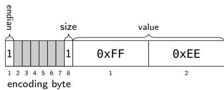
Figure 9.29: two byte big-endian value 65,518
