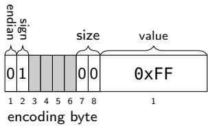
Figure 9.47: one byte little-endian value -255
