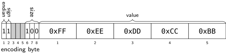
Figure 9.37: five byte big-endian value -1,099,224,173,755
