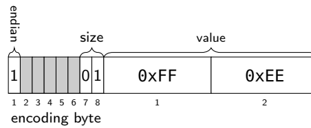
Figure 9.21: two byte big-endian value 65,518
