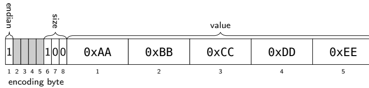
Figure 9.10: Dwm::EncodedU64 example: value 0xAABBCCDDEE, big-endian.
