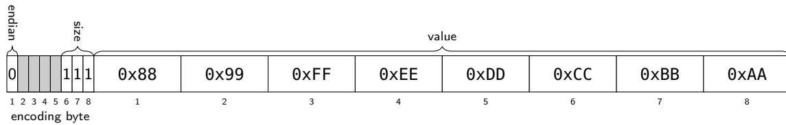
Figure 9.17: Dwm::EncodedU64 example: value 0xAABBCCDDEEFF9988, little-endian.
