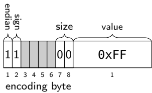
Figure 9.46: one byte big-endian value -255
