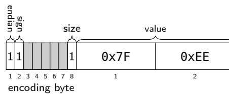
Figure 9.55: two byte big-endian value -32,750
