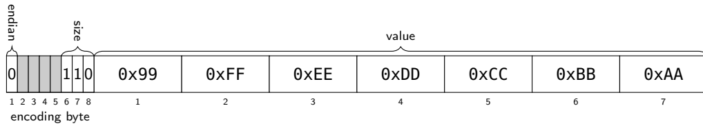
Figure 9.15: Dwm::EncodedU64 example: value 0xAABBCCDDEEFF99, little-endian.
