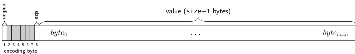
Figure 9.25: Dwm::EncodedU16 encoding
