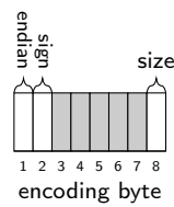
Figure 9.52: Encoding byte
