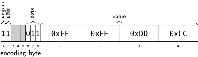
Figure 9.35: four byte big-endian value -4,293,844,428
