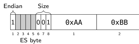
Figure 9.4: Two byte value 0xAABB, big-endian.
