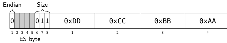
Figure 9.9: Four byte value 0xAABBCCDD, little-endian.
