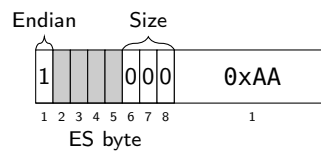
Figure 9.2: One byte value 0xAA, big-endian.
