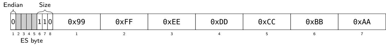
Figure 9.15: Seven byte value 0xAABBCCDDEEFF99, little-endian.
