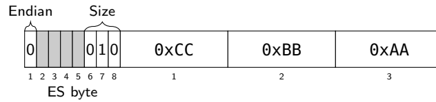
Figure 9.7: Three byte value 0xAABBCC, little-endian.
