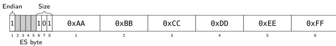
Figure 9.12: Six byte value 0xAABBCCDDEEFF, big-endian.
