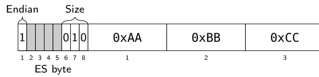
Figure 9.6: Three byte value 0xAABBCC, big-endian.
