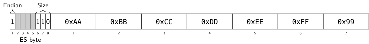
Figure 9.14: Seven byte value 0xAABBCCDDEEFF99, big-endian.
