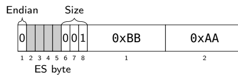
Figure 9.5: Two byte value 0xAABB, little-endian.
