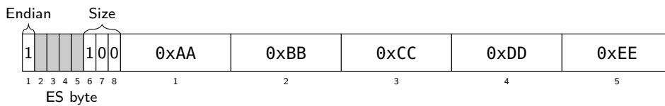
Figure 9.10: Five byte value 0xAABBCCDDEE, big-endian.
