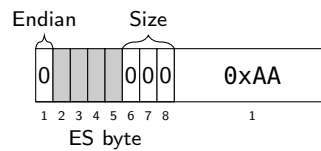
Figure 9.3: One byte value 0xAA, little-endian.
