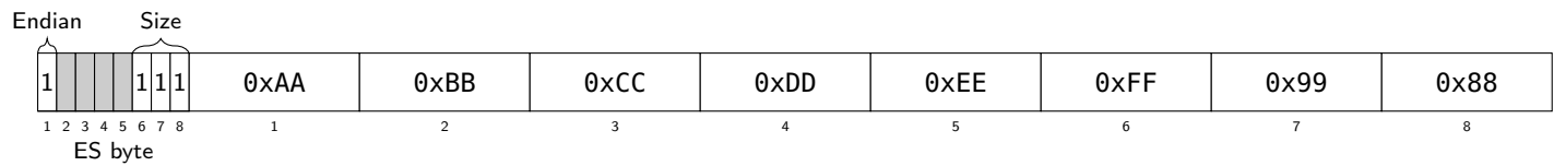
Figure 9.16: Eight byte value 0xAABBCCDDEEFF9988, big-endian.
