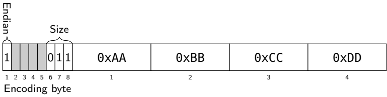
Figure 9.9: Four byte value 0xAABBCCDD, big-endian.
