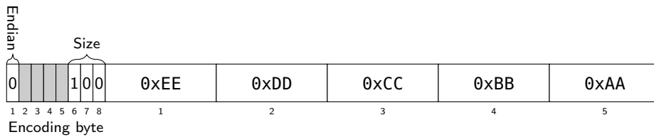
Figure 9.12: Five byte value 0xAABBCCDDEE, little-endian.
