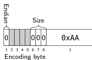
Figure 9.4: One byte value 0xAA, little-endian.
