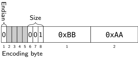
Figure 9.6: Two byte value 0xAABB, little-endian.
