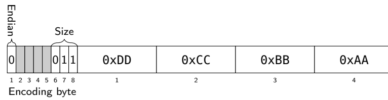
Figure 9.10: Four byte value 0xAABBCCDD, little-endian.
