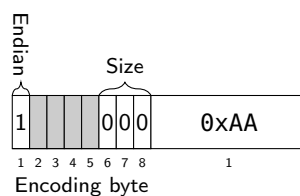
Figure 9.3: One byte value 0xAA, big-endian.
