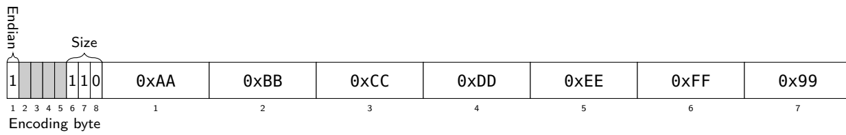
Figure 9.15: Seven byte value 0xAABBCCDDEEFF99, big-endian.
