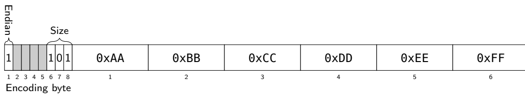
Figure 9.13: Six byte value 0xAABBCCDDEEFF, big-endian.
