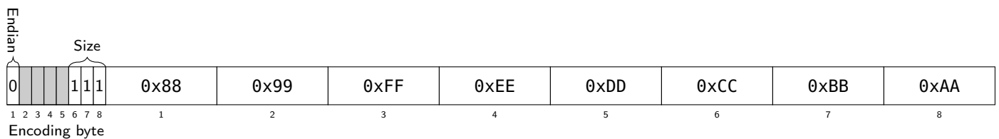
Figure 9.18: Eight byte value 0xAABBCCDDEEFF9988, little-endian.
