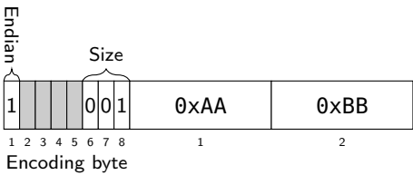
Figure 9.5: Two byte value 0xAABB, big-endian.
