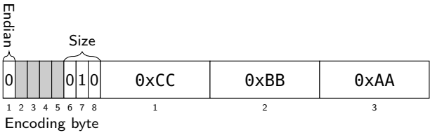
Figure 9.8: Three byte value 0xAABBCC, little-endian.
