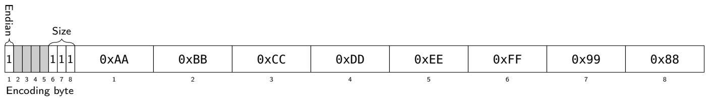
Figure 9.17: Eight byte value 0xAABBCCDDEEFF9988, big-endian.
