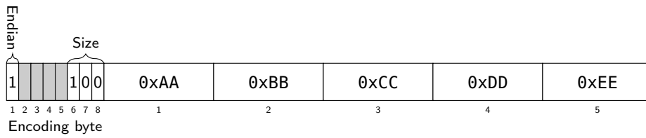
Figure 9.11: Five byte value 0xAABBCCDDEE, big-endian.
