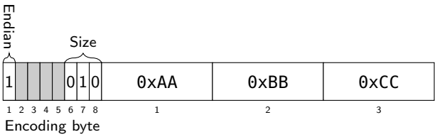
Figure 9.7: Three byte value 0xAABBCC, big-endian.
