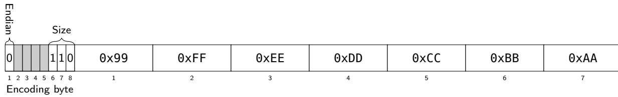
Figure 9.16: Seven byte value 0xAABBCCDDEEFF99, little-endian.
