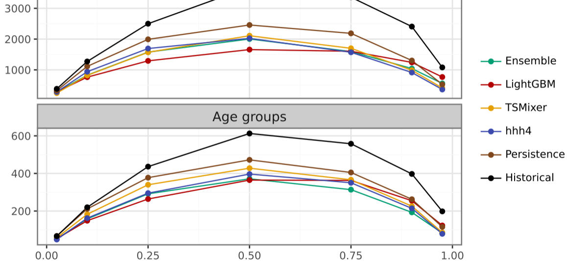
Quantile level
