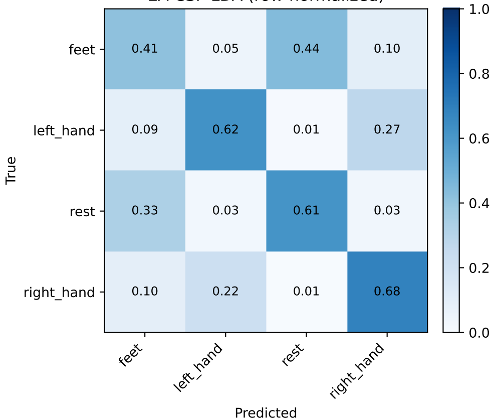
EA-CSP-LDA (row-normalized)
