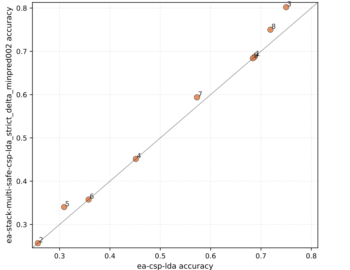
Per-subject accuracy: ea-csp-lda vs ea-stack-multi-safe-csp-lda_strict_delta_minpred002 ( \Delta mean=+0.015, +4/05/-0)
