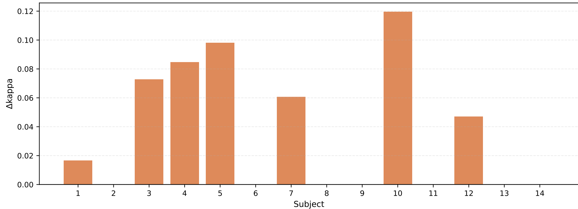
Per-subject \Delta kappa: ea-fbcsp-pred-disagree-safe – ea-csp-lda ( \Delta mean=+0.036)
