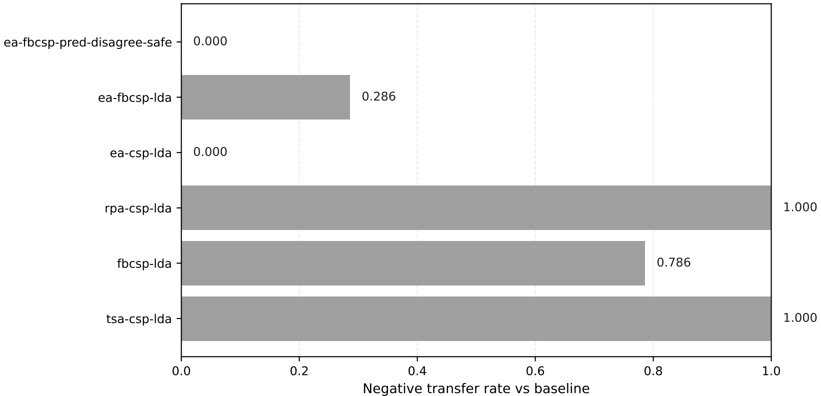
Schirrmeister2017 LOSO-4class (0train, rs=50): negative transfer rate vs EA (lower is better)
