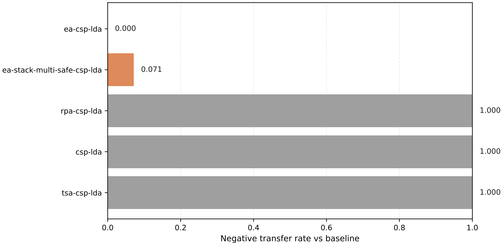
LOSO-4class: negative transfer rate vs EA (lower is better)
