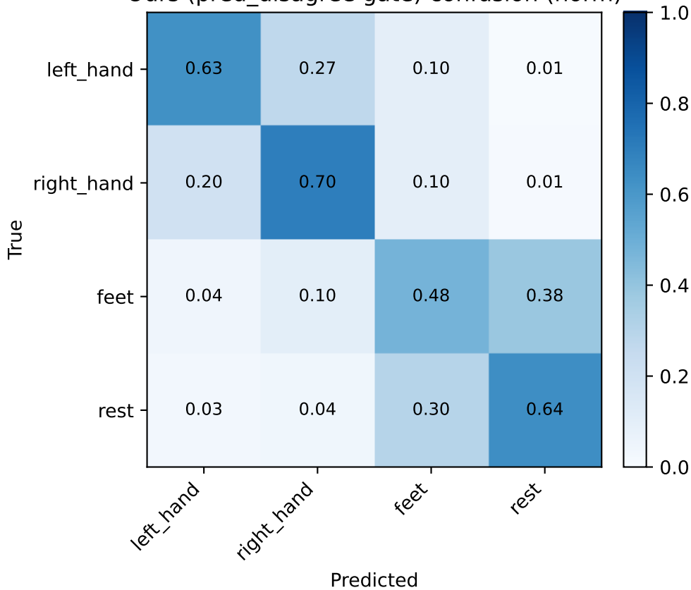
Ours (pred_disagree gate) confusion (norm)
