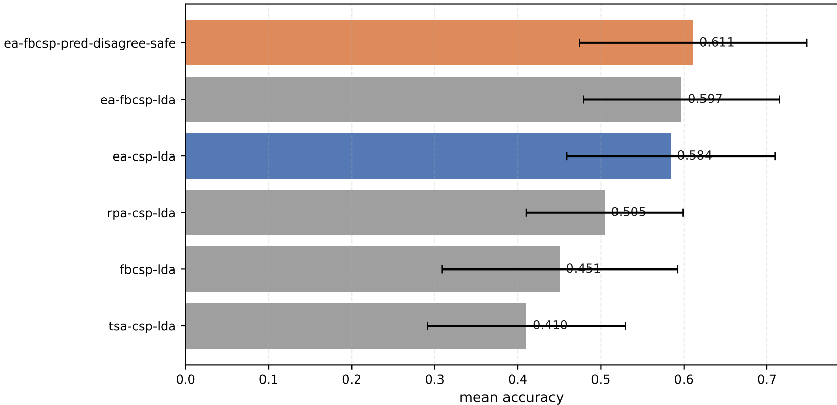
Schirrmeister2017 LOSO-4class (0train, rs=50): mean accuracy ( \pm std across subjects)
