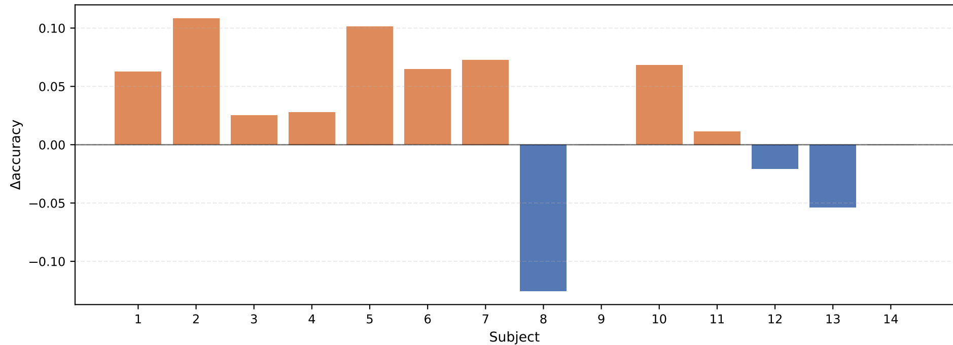
Per-subject \Delta accuracy: ea-stack-multi-safe-csp-lda – ea-csp-lda ( \Delta mean=+0.024)
