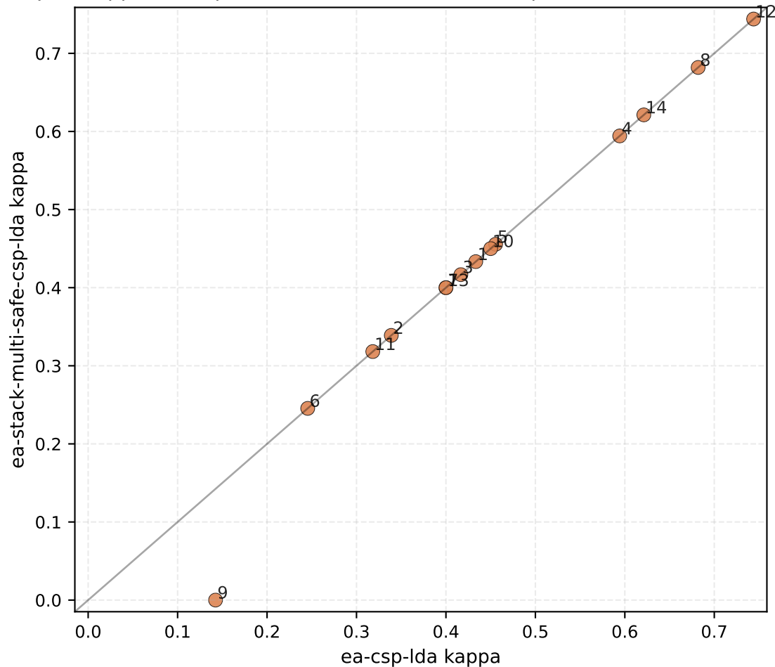
Per-subject kappa: ea-csp-lda vs ea-stack-multi-safe-csp-lda ( \Delta\text{mean}=-0.010 , +0/013/-1 )
