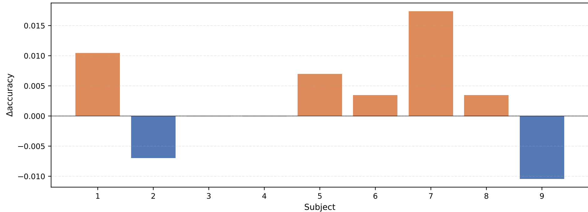
Per-subject \Delta accuracy: lea-csp-lda – ea-csp-lda ( \Delta mean=+0.003)
