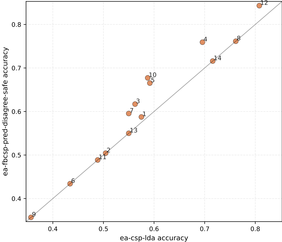
Per-subject accuracy: ea-csp-lda vs ea-fbcsp-pred-disagree-safe ( \Delta\text{mean} = +0.027, +7/07/-0 )
