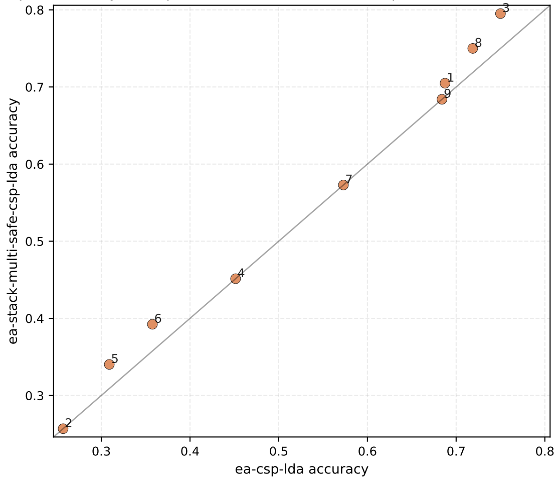
Per-subject accuracy: ea-csp-lda vs ea-stack-multi-safe-csp-lda ( \Delta\text{mean} = +0.018 , +5/04/-0)
