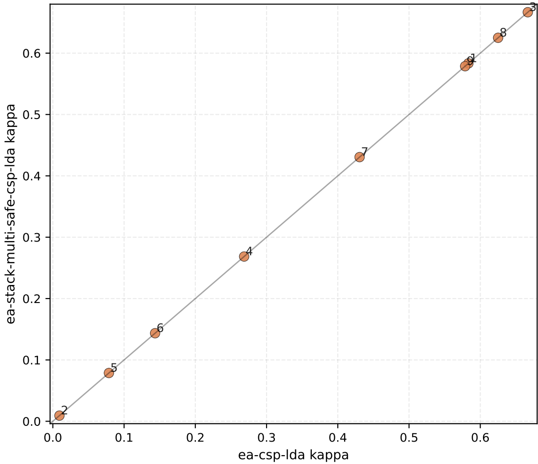
Per-subject kappa: ea-csp-lda vs ea-stack-multi-safe-csp-lda ( \Delta\text{mean} = +0.000 , +0/09/-0 )
