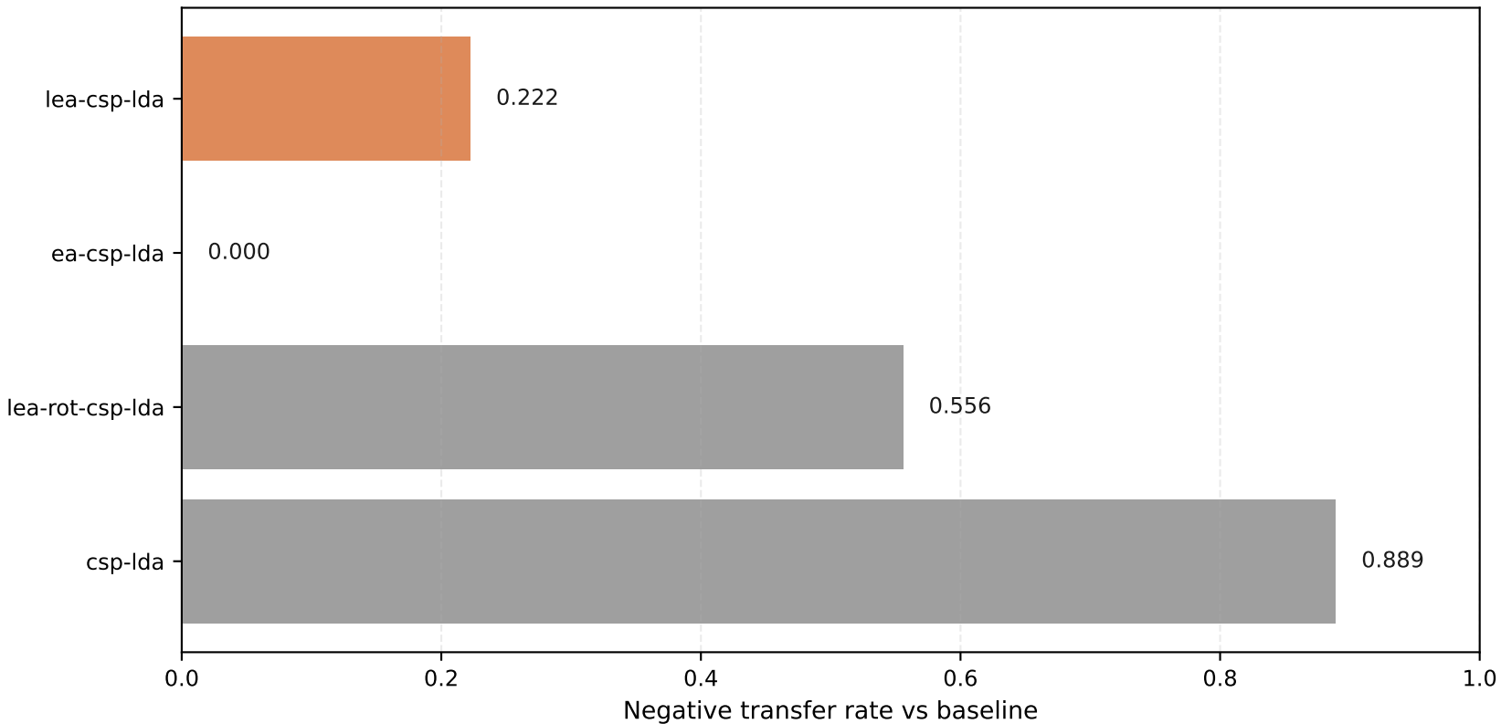
BNCI2014_001 CrossSession 0train→1test (4-class): negative transfer rate vs EA (lower is better)
