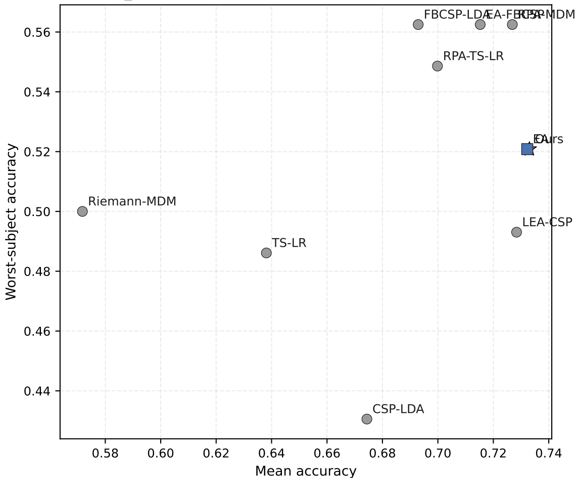
BNCI2014_001 LOSO-2class (strict): mean vs worst-subject accuracy
