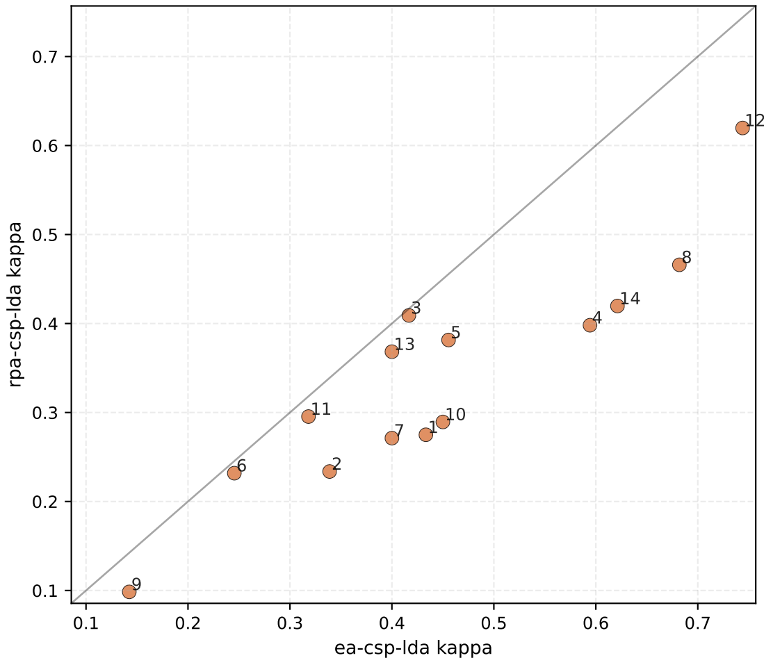
Per-subject kappa: ea-csp-lda vs rpa-csp-lda ( \Delta\text{mean}=-0.106 , +0/00/-14 )
