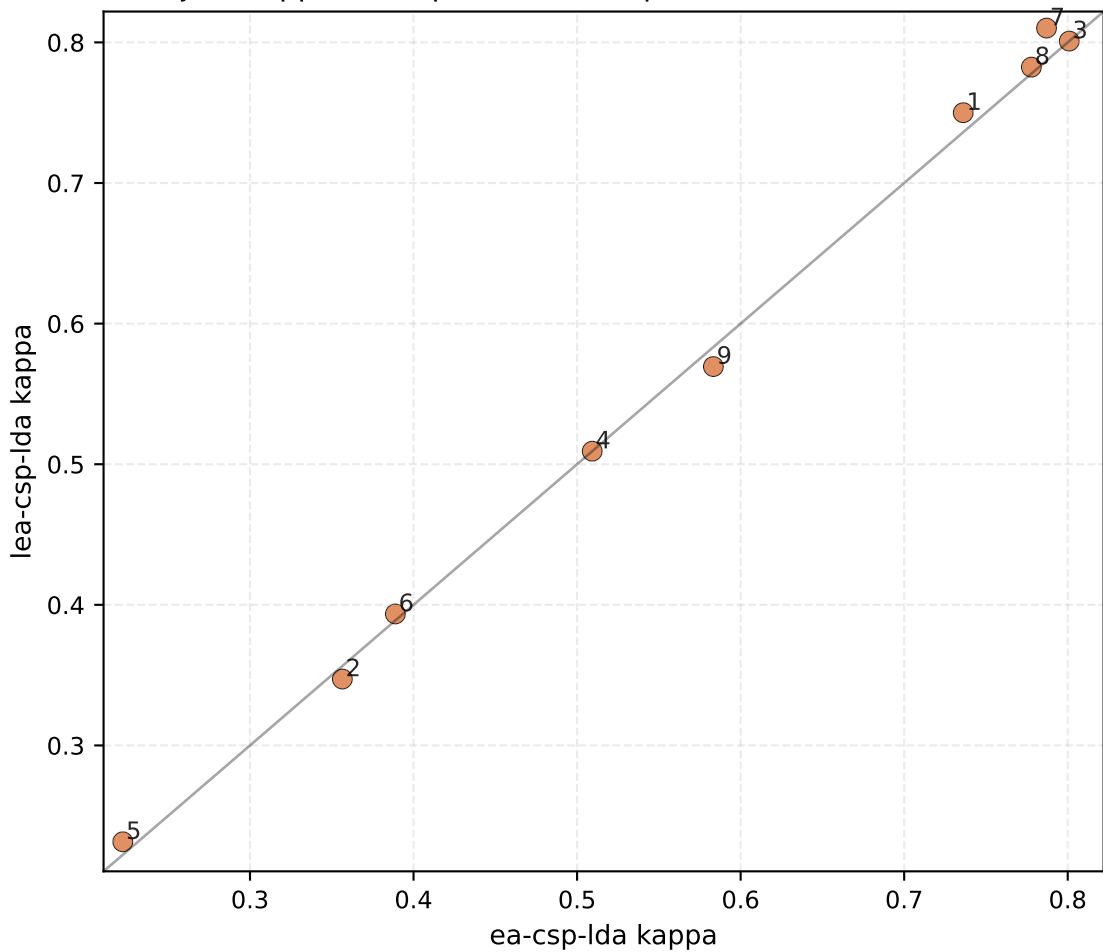
Per-subject kappa: ea-csp-lda vs lea-csp-lda ( \Delta\text{mean} = +0.004, +5/02/-2 )
