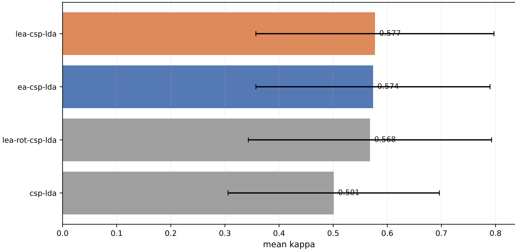
BNCI2014_001 CrossSession 0train→1test (4-class): mean kappa ( \pm std across subjects)
