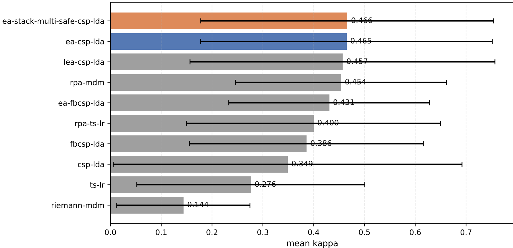
BNCI2014_001 LOSO-2class (strict): mean kappa ( \pm std across subjects)
