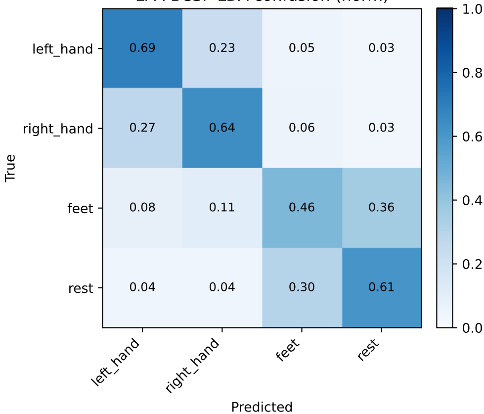
EA-FBCSP-LDA confusion (norm)
