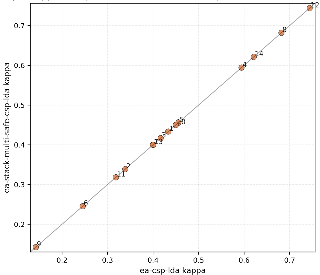
Per-subject kappa: ea-csp-lda vs ea-stack-multi-safe-csp-lda ( \Delta\text{mean} = +0.000, +0/014/-0 )
