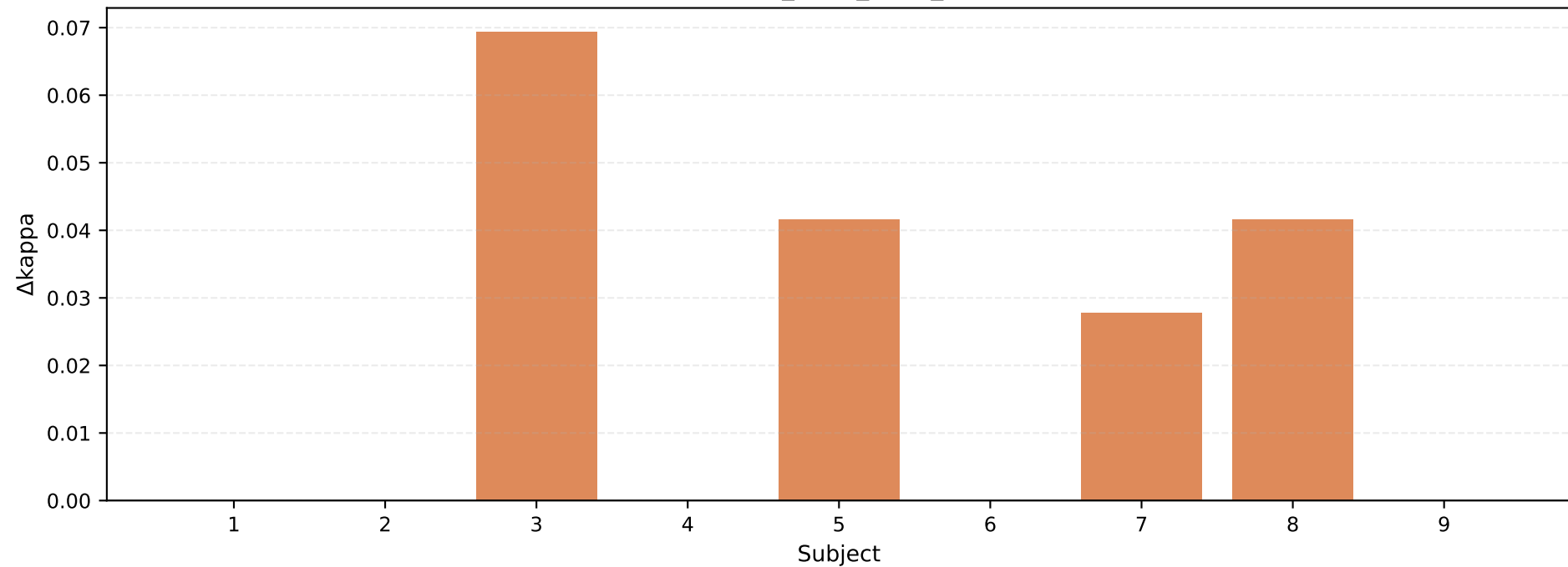
Per-subject \Delta\kappa : ea-stack-multi-safe-csp-lda_strict_delta_minpred002 – ea-csp-lda ( \Delta\text{mean}=+0.020 )
