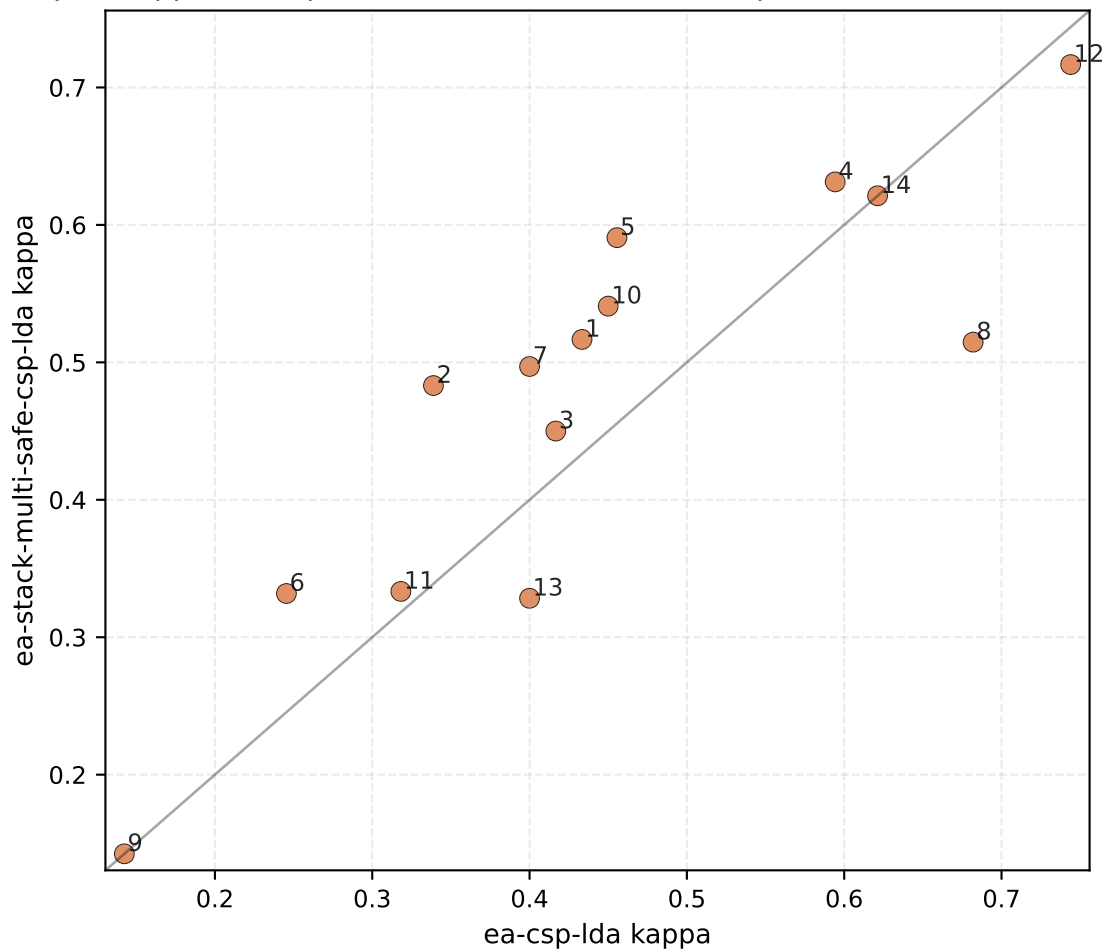
Per-subject kappa: ea-csp-lda vs ea-stack-multi-safe-csp-lda ( \Delta\text{mean} = +0.033 , +9/02/-3 )
