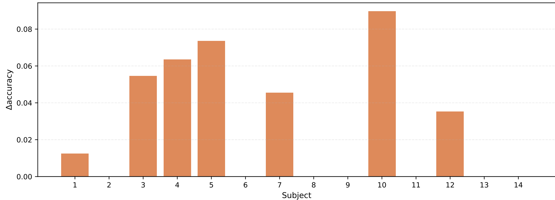
Per-subject \Delta accuracy: ea-fbcsp-pred-disagree-safe – ea-csp-lda ( \Delta mean=+0.027)
