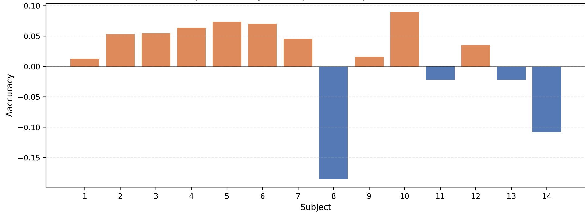
Per-subject \Delta accuracy: ea-fbcsp-lda – ea-csp-lda ( \Delta mean=+0.013)
