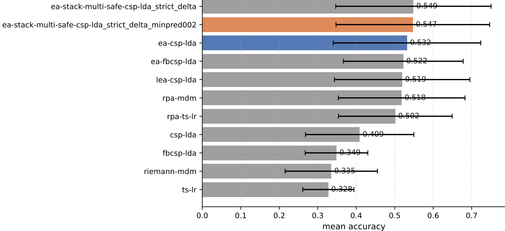
LOSO-4class: mean accuracy ( \pm std across subjects)
