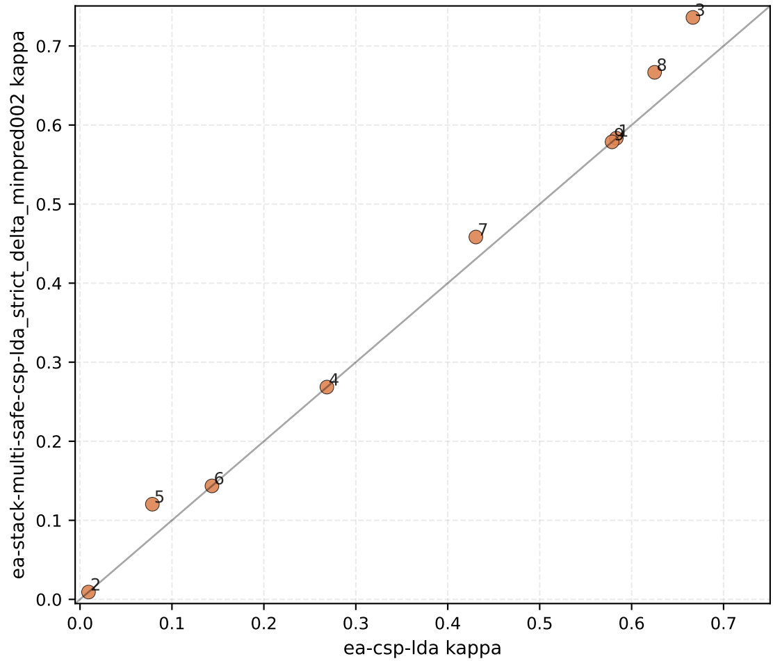
Per-subject kappa: ea-csp-lda vs ea-stack-multi-safe-csp-lda_strict_delta_minpred002 ( \Delta\text{mean} = +0.020 , +4/05/-0)
