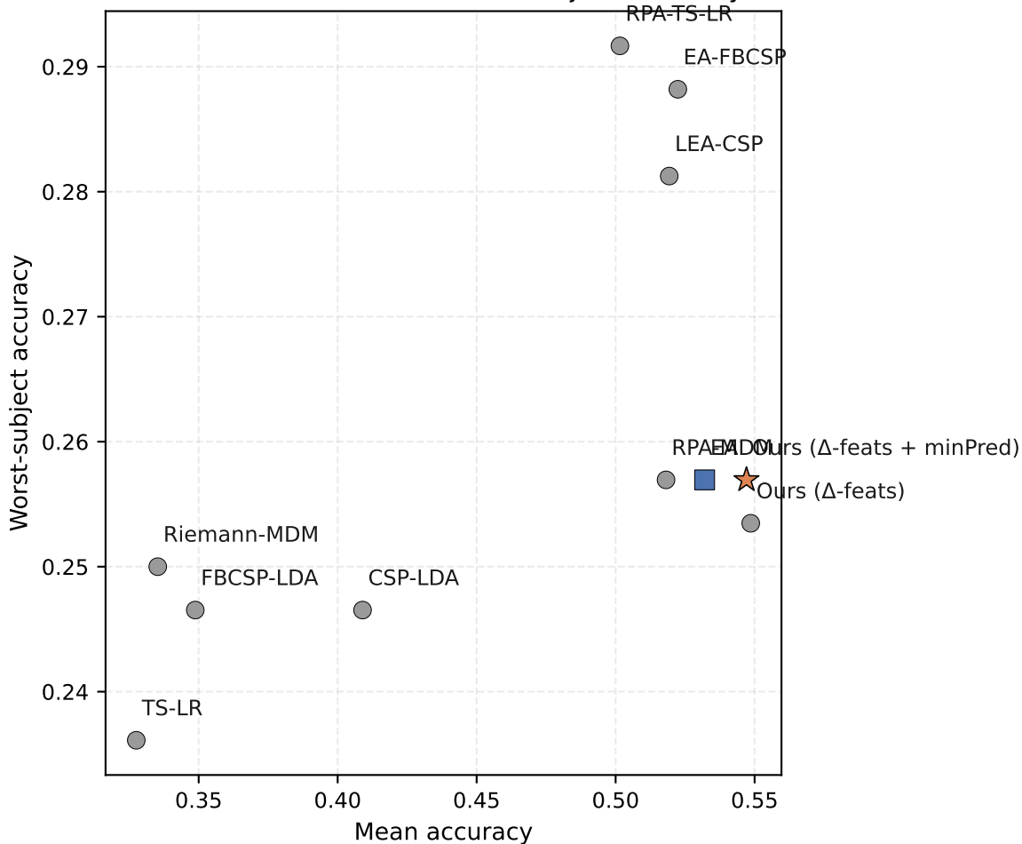
LOSO-4class: mean vs worst-subject accuracy
