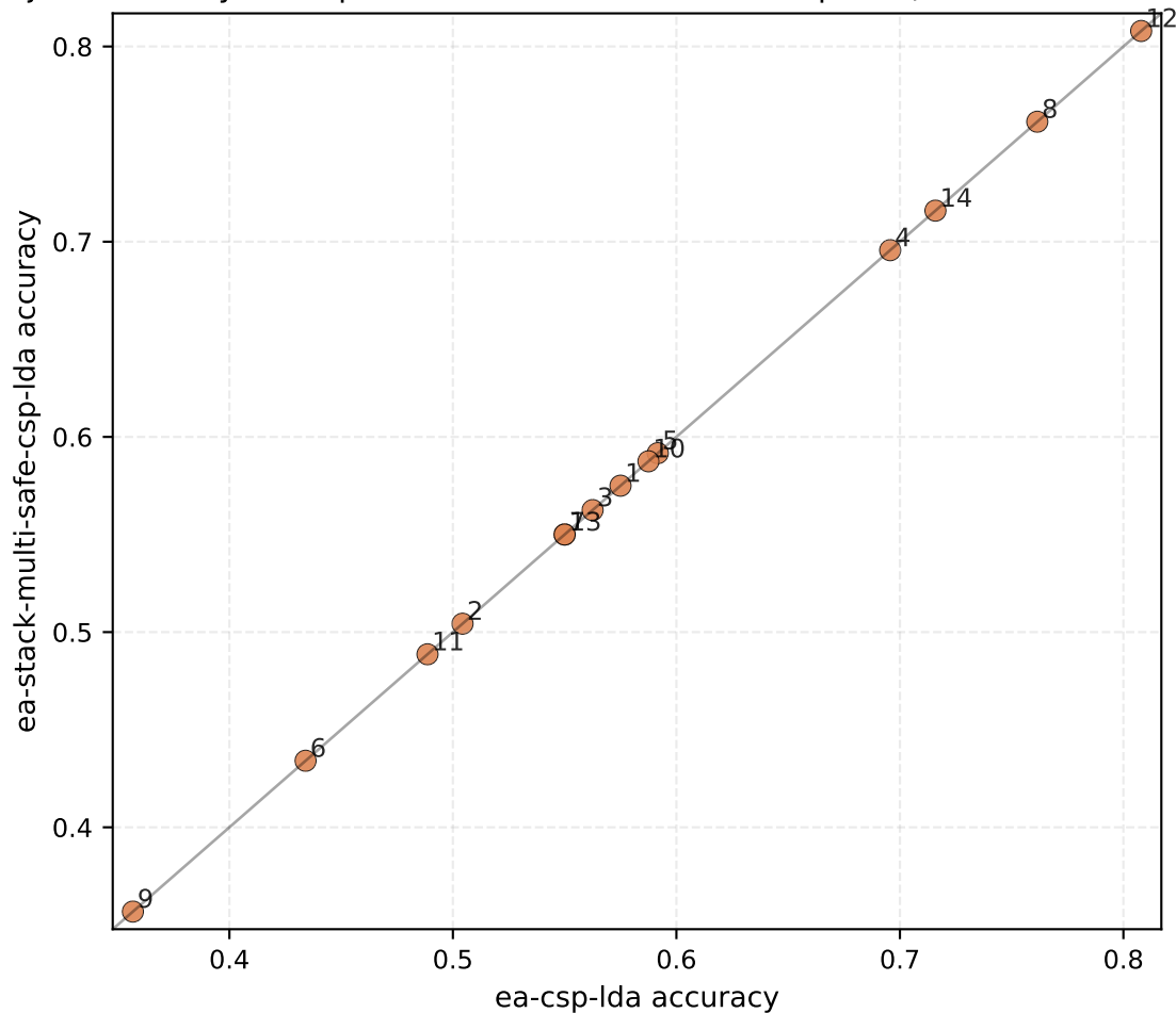
Per-subject accuracy: ea-csp-lda vs ea-stack-multi-safe-csp-lda ( \Delta\text{mean} = +0.000, +0/014/-0 )
