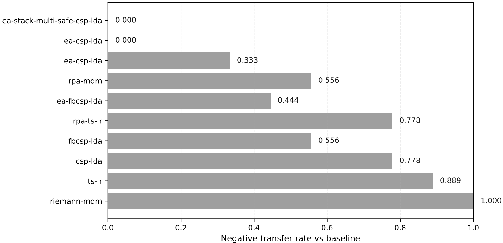
BNCI2014_001 LOSO-2class (strict): negative transfer rate vs EA (lower is better)
