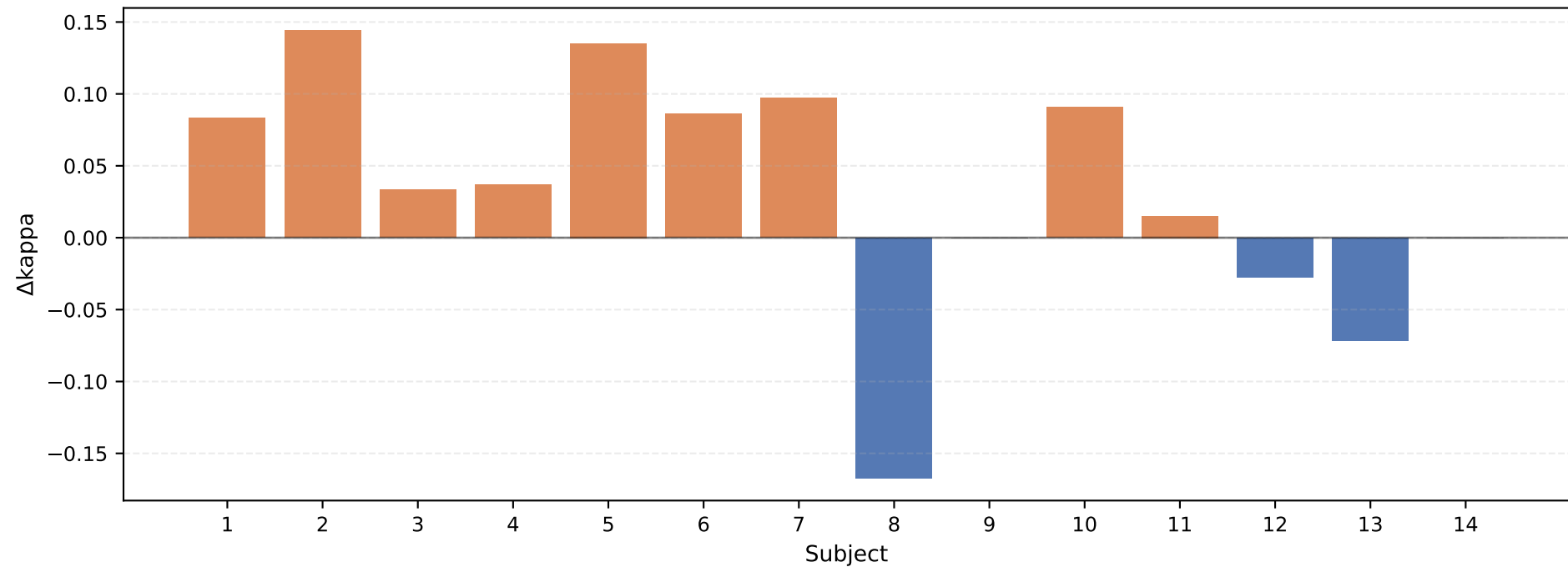
Per-subject \Delta kappa: ea-stack-multi-safe-csp-lda – ea-csp-lda ( \Delta mean=+0.033)
