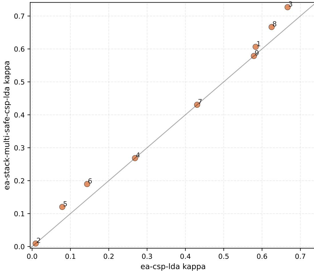
Per-subject kappa: ea-csp-lda vs ea-stack-multi-safe-csp-lda ( \Delta\text{mean} = +0.024 , +5/04/-0 )
