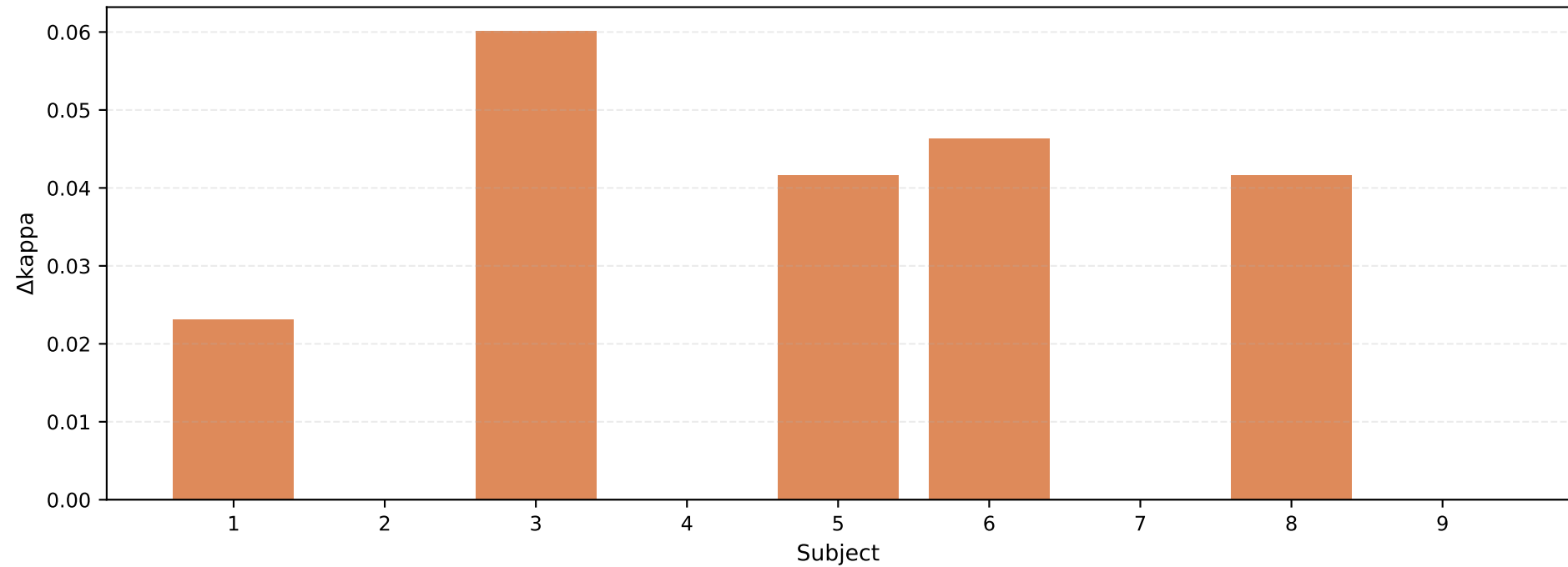
Per-subject \Delta\kappa : ea-stack-multi-safe-csp-lda – ea-csp-lda ( \Delta\text{mean}=+0.024 )
