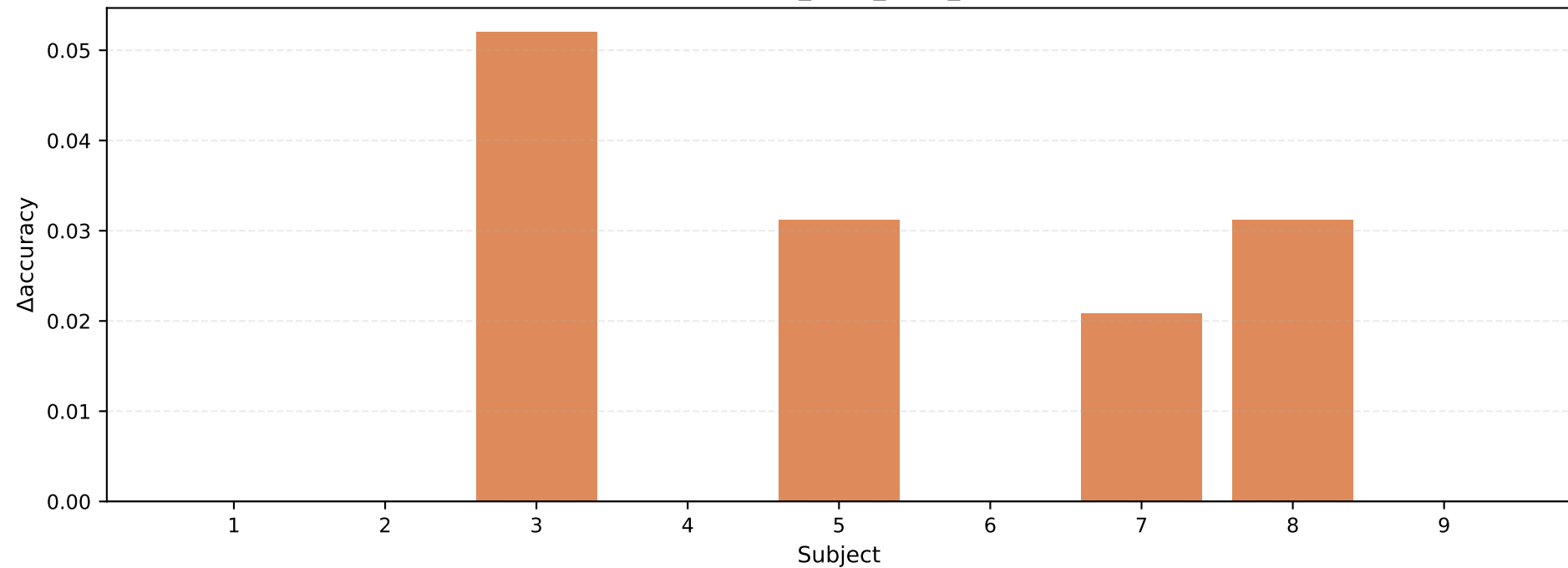
Per-subject \Delta accuracy: ea-stack-multi-safe-csp-lda_strict_delta_minpred002 – ea-csp-lda ( \Delta mean=+0.015)
