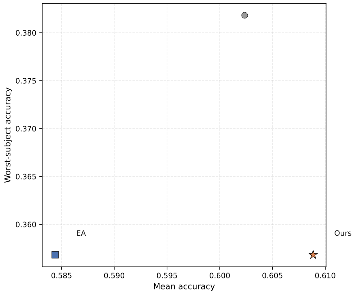
Schirrmeister2017 LOSO-4class (0train, rs=50): mean vs worst-subject accuracy
