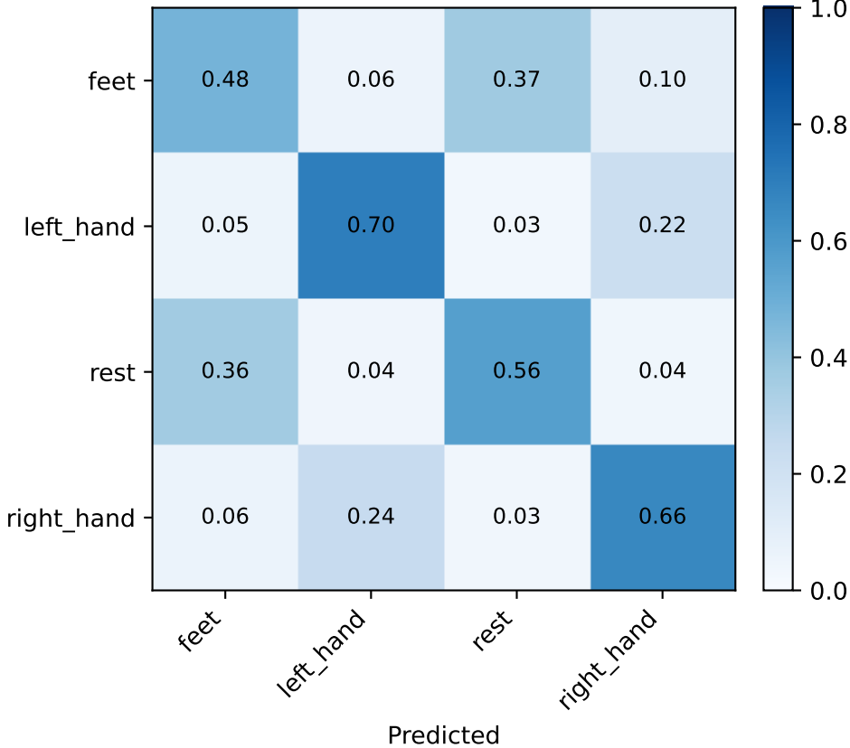
EA-FBCSP-LDA (row-normalized)
