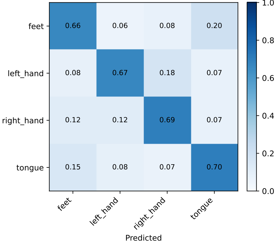
EA-CSP-LDA (row-normalized)
