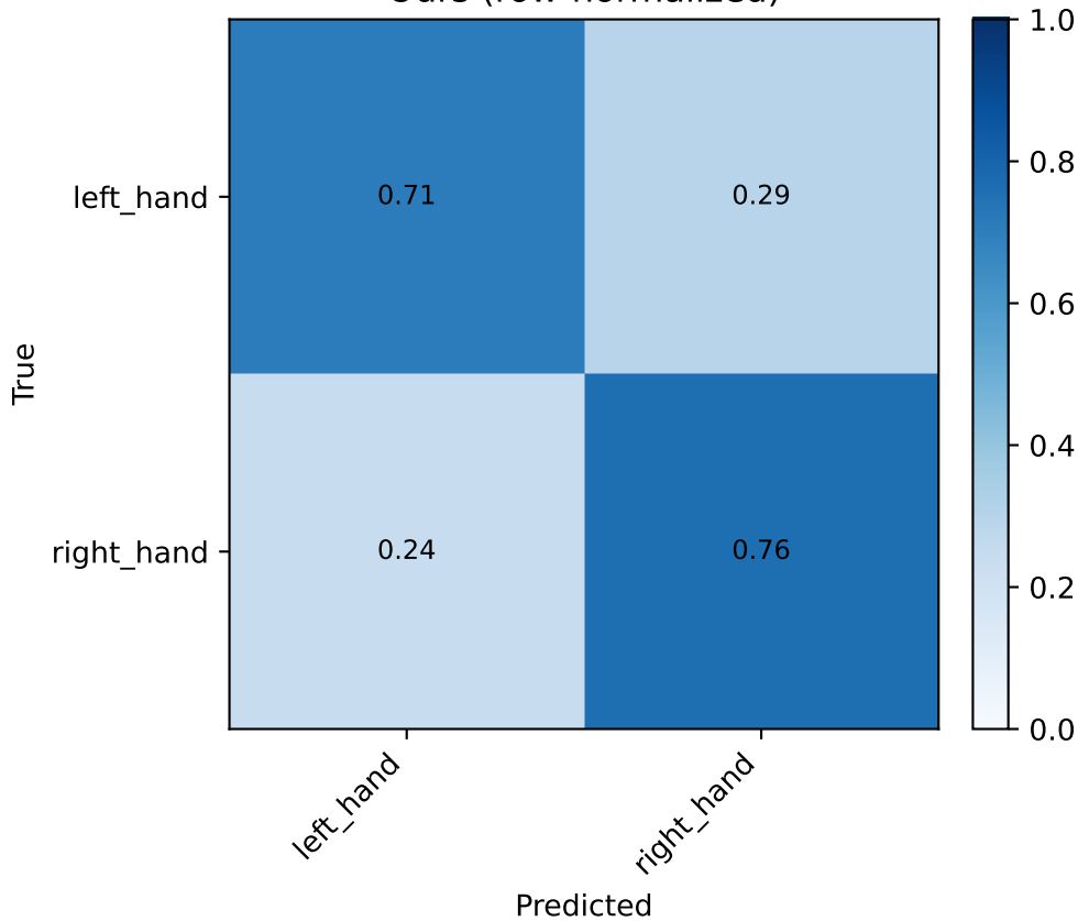
Ours (row-normalized)
