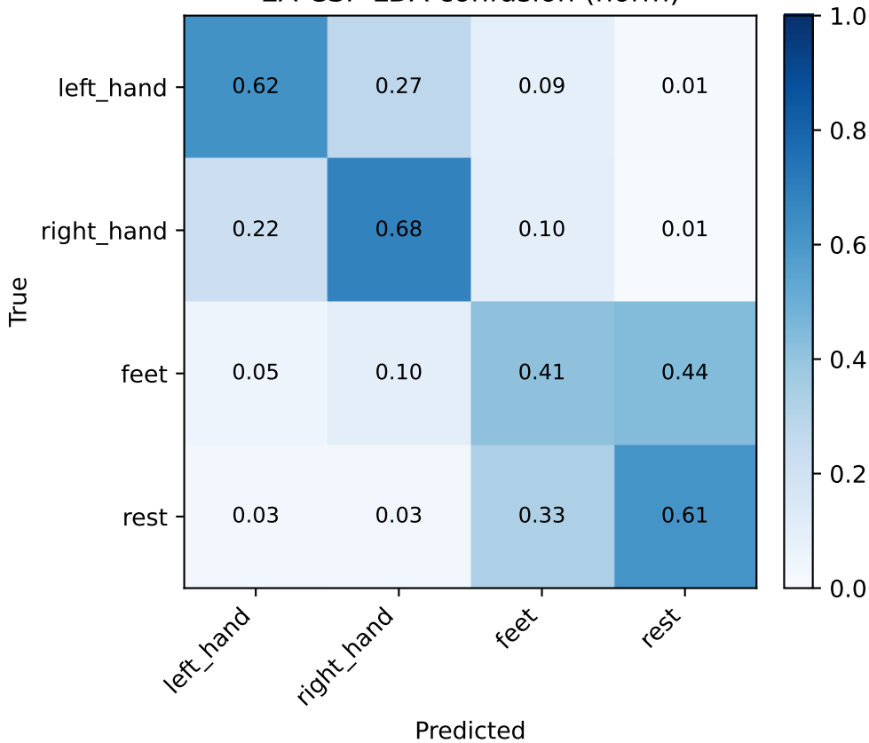
EA-CSP-LDA confusion (norm)
