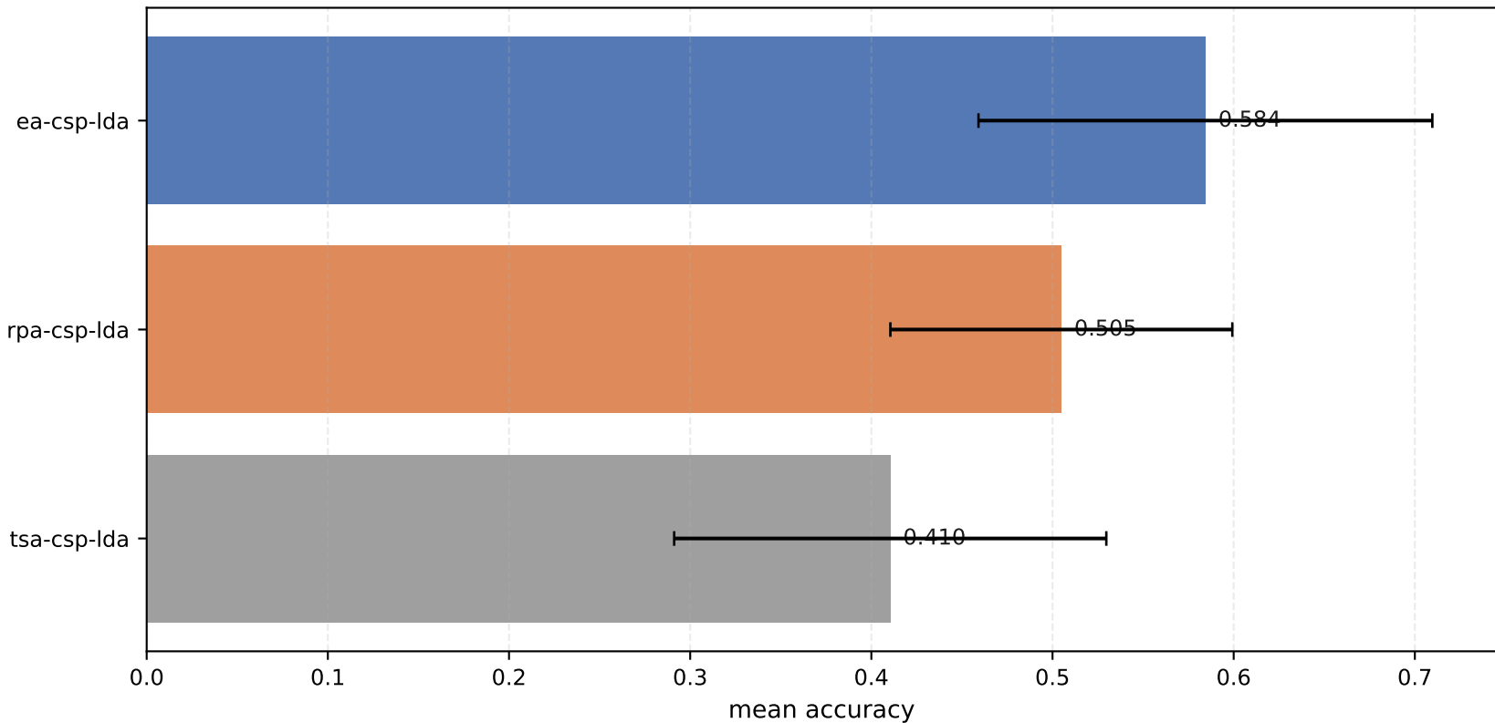
LOSO-4class: mean accuracy ( \pm std across subjects)
