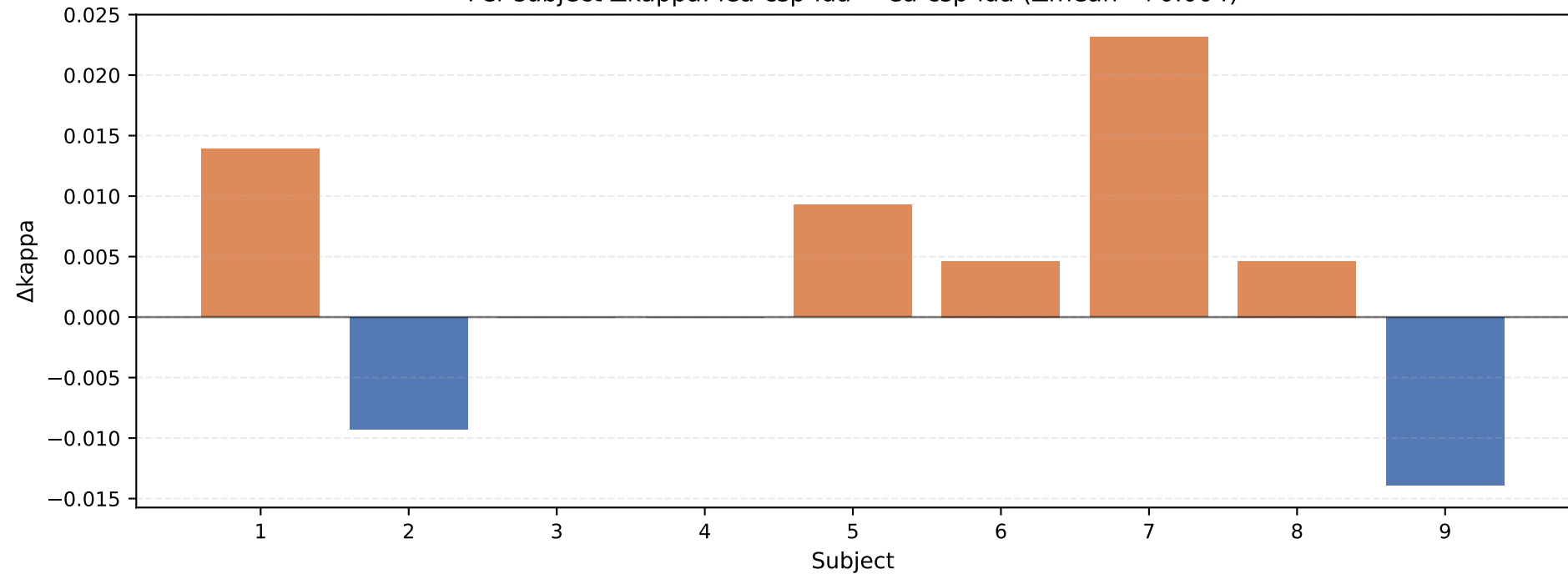
Per-subject \Delta kappa: lea-csp-lda – ea-csp-lda ( \Delta mean=+0.004)
