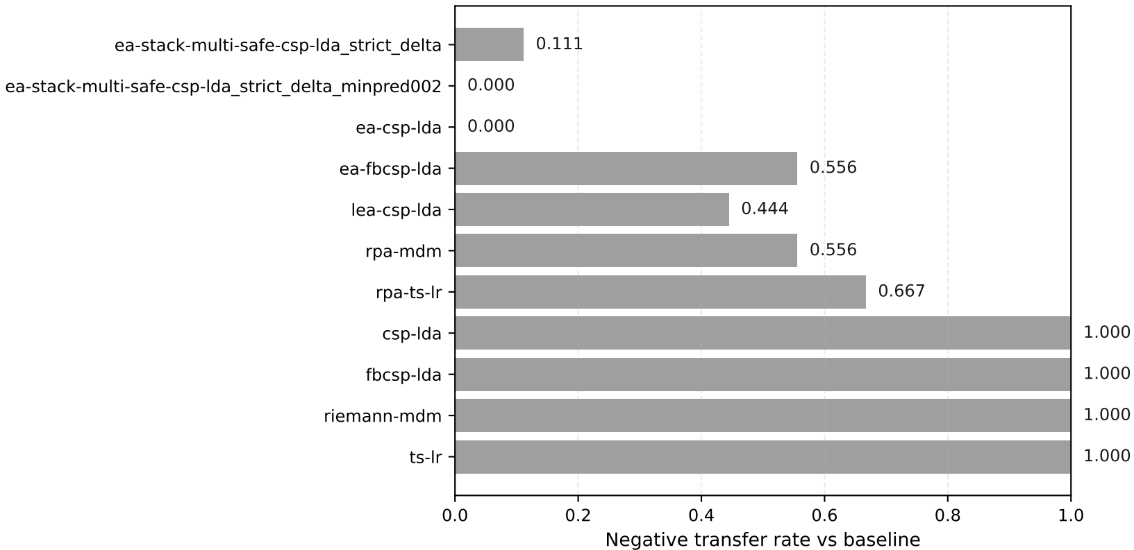
LOSO-4class: negative transfer rate vs EA (lower is better)
