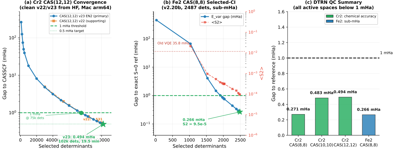
FIG. 9. DTRN quantum chemistry benchmarks. (a) Cr 2 CAS(12,12) convergence with v23 EN2-selected CI (primary) and v22 residual-selected CI (supporting), both started from the HF determinant. Star: v23 headline (0.494 mHa, 102,001 dets, 19.5 min). The 1 mHa threshold is crossed at 75,001 determinants (14.9 min); the 0.5 mHa target at 102,001 determinants (19.5 min). (b) Fe 2 CAS(8,8) v2.20b: gap (left) and \langle S^2 \rangle (right) decrease together; sub-mHa at 2,487 determinants. (c) Summary: all four active spaces achieve sub-mHa or < 1 mHa accuracy.
