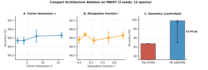
FIG. 5. Compact architecture ablation on mnist (3 seeds, 12 epochs) . Left: d -sweep—accuracy is flat across matched-width settings, with the wider ( d=8 , k=3 , N=512 ) control giving comparable performance, confirming logarithmic-scaling robustness. Centre: f -sweep—performance is insensitive to dissipation fraction across the full tested range. Right: geometry axis—PE-GADTRN vs. flat at identical backbone; the 12.64 pp gap directly quantifies the geometry contribution.
