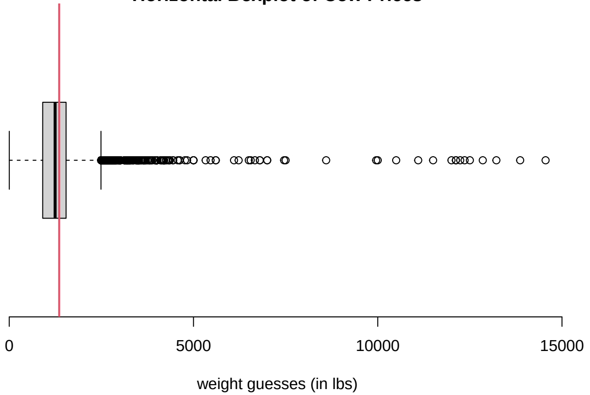
Horizontal Boxplot of Cow Prices
